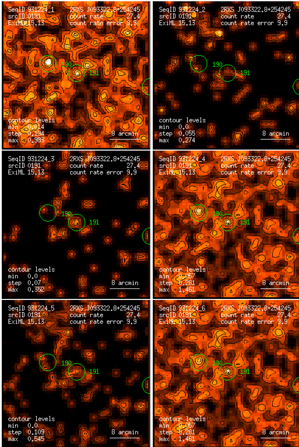
Figure 191: RASS 931224: detection 0191: band rate images, Gaussian filter: (1) PSPC channels 11 – 41, (2) 52 – 90, (3) 91 – 201, (4) 11 – 235, (5) 52 – 201, (6) 11 – 201. Broad band rates in counts/ks. Band rate contour levels in counts/ks/arcmin 2 .
