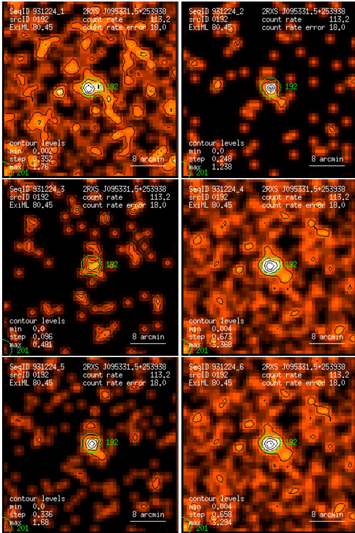
Figure 192: RASS 931224: detection 0192: band rate images, Gaussian filter: (1) PSPC channels 11 – 41, (2) 52 – 90, (3) 91 – 201, (4) 11 – 235, (5) 52 – 201, (6) 11 – 201. Broad band rates in counts/ks. Band rate contour levels in counts/ks/arcmin 2 .
