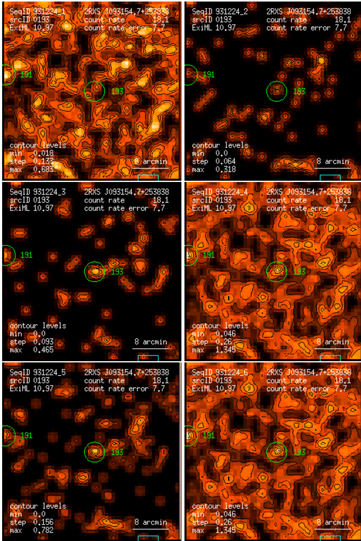
Figure 193: RASS 931224: detection 0193: band rate images, Gaussian filter: (1) PSPC channels 11 – 41, (2) 52 – 90, (3) 91 – 201, (4) 11 – 235, (5) 52 – 201, (6) 11 – 201. Broad band rates in counts/ks. Band rate contour levels in counts/ks/arcmin 2 .
