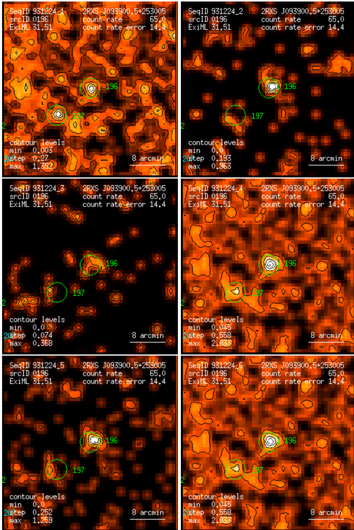
Figure 196: RASS 931224: detection 0196: band rate images, Gaussian filter: (1) PSPC channels 11 – 41, (2) 52 – 90, (3) 91 – 201, (4) 11 – 235, (5) 52 – 201, (6) 11 – 201. Broad band rates in counts/ks. Band rate contour levels in counts/ks/arcmin 2 .
