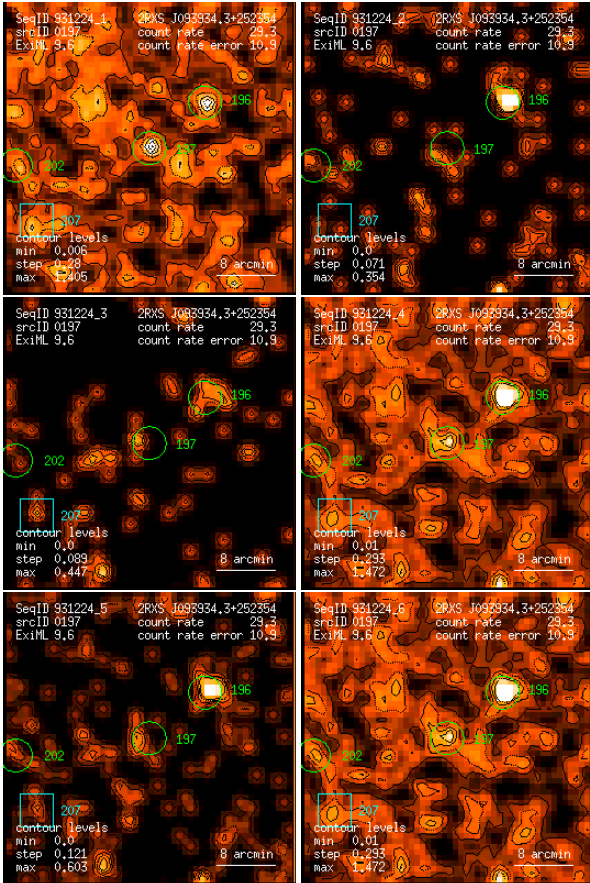
Figure 197: RASS 931224: detection 0197: band rate images, Gaussian filter: (1) PSPC channels 11 – 41, (2) 52 – 90, (3) 91 – 201, (4) 11 – 235, (5) 52 – 201, (6) 11 – 201. Broad band rates in counts/ks. Band rate contour levels in counts/ks/arcmin 2 .
