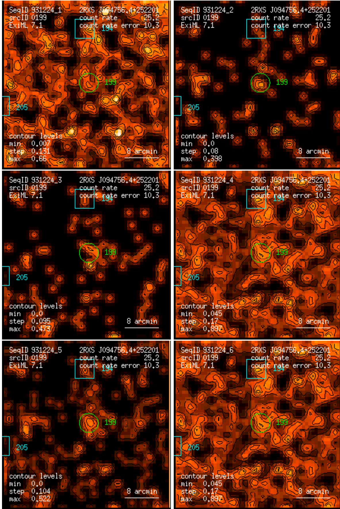
Figure 199: RASS 931224: detection 0199: band rate images, Gaussian filter: (1) PSPC channels 11 – 41, (2) 52 – 90, (3) 91 – 201, (4) 11 – 235, (5) 52 – 201, (6) 11 – 201. Broad band rates in counts/ks. Band rate contour levels in counts/ks/arcmin 2 .
