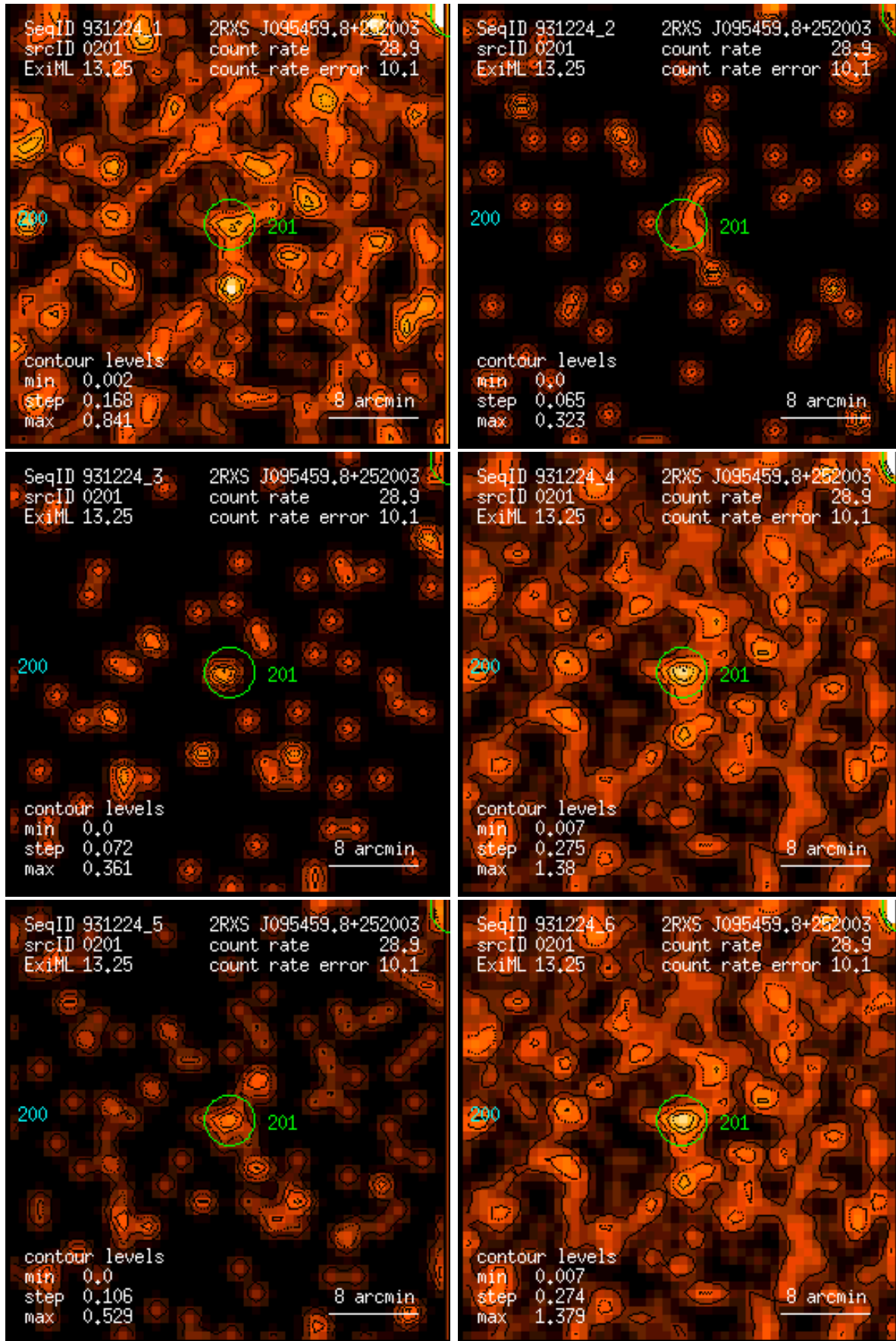
Figure 201: RASS 931224: detection 0201: band rate images, Gaussian filter: (1) PSPC channels 11 – 41, (2) 52 – 90, (3) 91 – 201, (4) 11 – 235, (5) 52 – 201, (6) 11 – 201. Broad band rates in counts/ks. Band rate contour levels in counts/ks/arcmin 2 .
