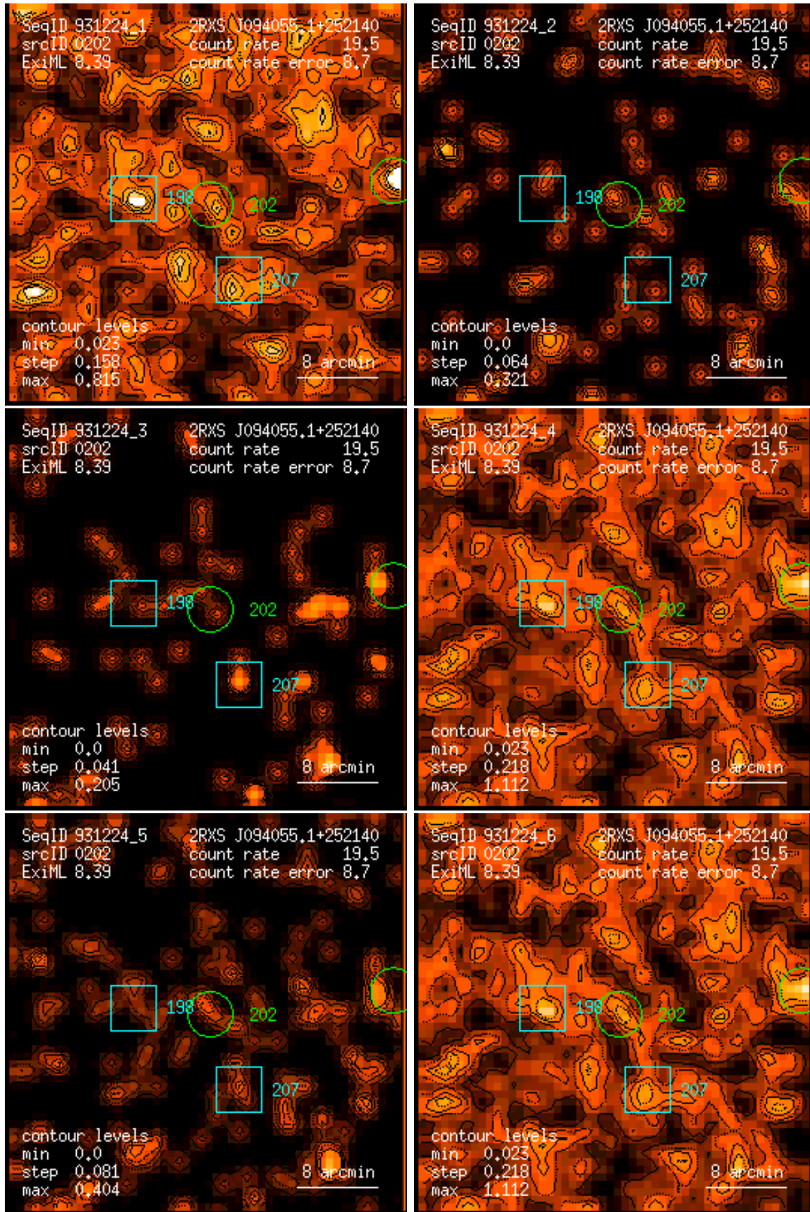
Figure 202: RASS 931224: detection 0202: band rate images, Gaussian filter: (1) PSPC channels 11 – 41, (2) 52 – 90, (3) 91 – 201, (4) 11 – 235, (5) 52 – 201, (6) 11 – 201. Broad band rates in counts/ks. Band rate contour levels in counts/ks/arcmin 2 .
