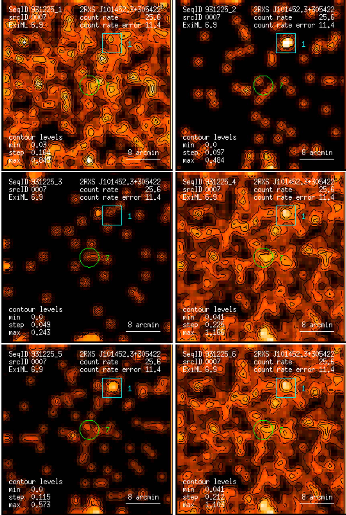
Figure 7: RASS 931225: detection 0007: band rate images, Gaussian filter: (1) PSPC channels 11 – 41, (2) 52 – 90, (3) 91 – 201, (4) 11 – 235, (5) 52 – 201, (6) 11 – 201. Broad band rates in counts/ks. Band rate contour levels in counts/ks/arcmin 2 .
