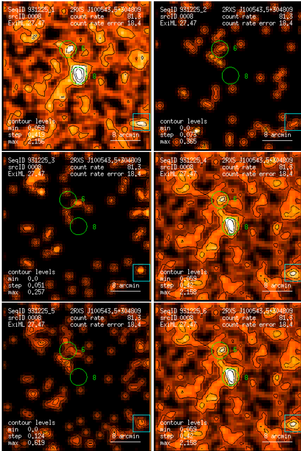
Figure 8: RASS 931225: detection 0008: band rate images, Gaussian filter: (1) PSPC channels 11 – 41, (2) 52 – 90, (3) 91 – 201, (4) 11 – 235, (5) 52 – 201, (6) 11 – 201. Broad band rates in counts/ks. Band rate contour levels in counts/ks/arcmin 2 .
