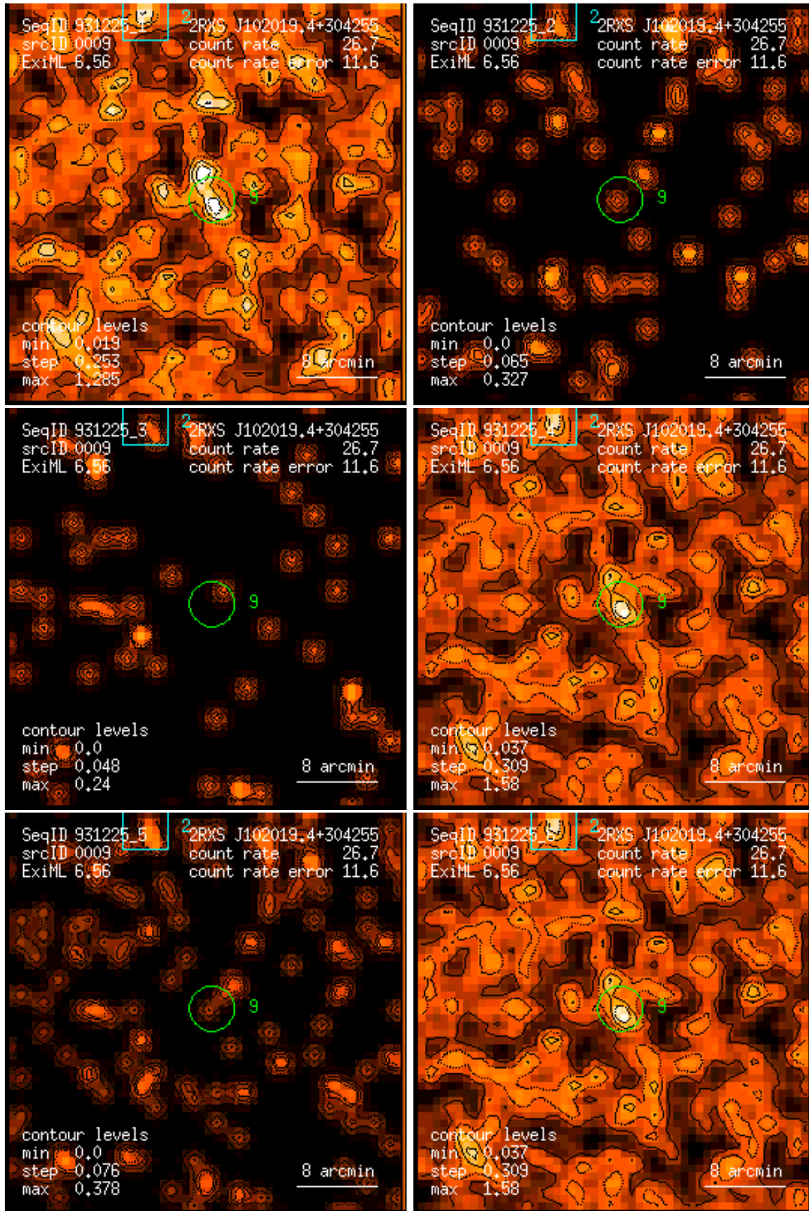
Figure 9: RASS 931225: detection 0009: band rate images, Gaussian filter: (1) PSPC channels 11 – 41, (2) 52 – 90, (3) 91 – 201, (4) 11 – 235, (5) 52 – 201, (6) 11 – 201. Broad band rates in counts/ks. Band rate contour levels in counts/ks/arcmin 2 .
