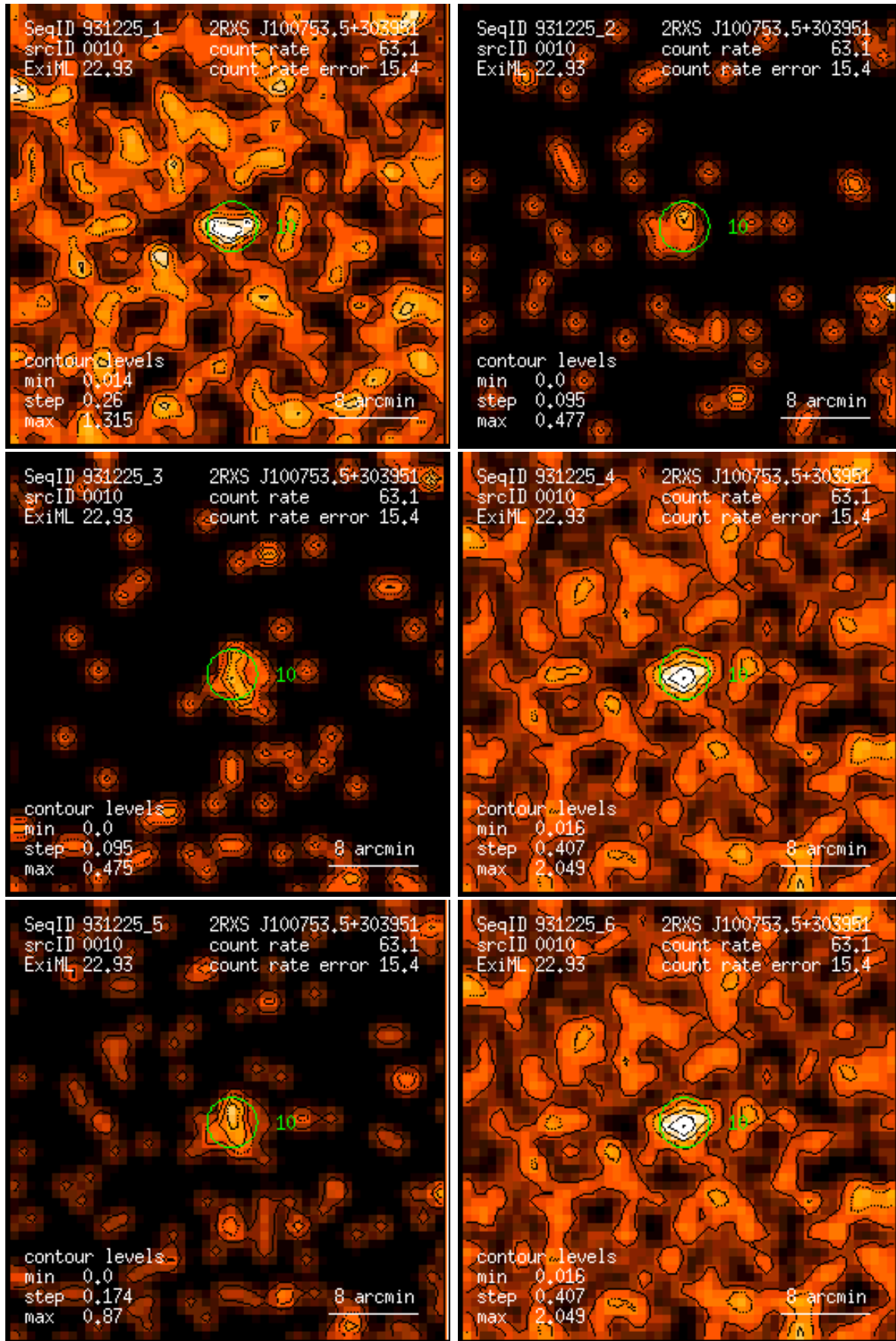
Figure 10: RASS 931225: detection 0010: band rate images, Gaussian filter: (1) PSPC channels 11 – 41, (2) 52 – 90, (3) 91 – 201, (4) 11 – 235, (5) 52 – 201, (6) 11 – 201. Broad band rates in counts/ks. Band rate contour levels in counts/ks/arcmin 2 .
