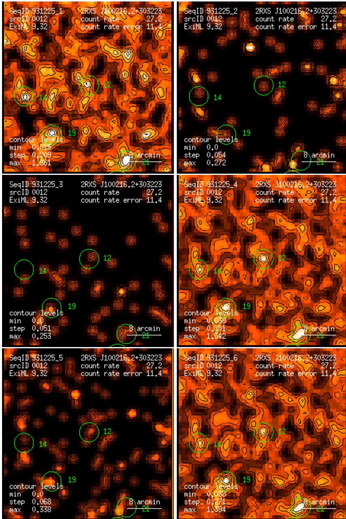
Figure 12: RASS 931225: detection 0012: band rate images, Gaussian filter: (1) PSPC channels 11 – 41, (2) 52 – 90, (3) 91 – 201, (4) 11 – 235, (5) 52 – 201, (6) 11 – 201. Broad band rates in counts/ks. Band rate contour levels in counts/ks/arcmin 2 .
