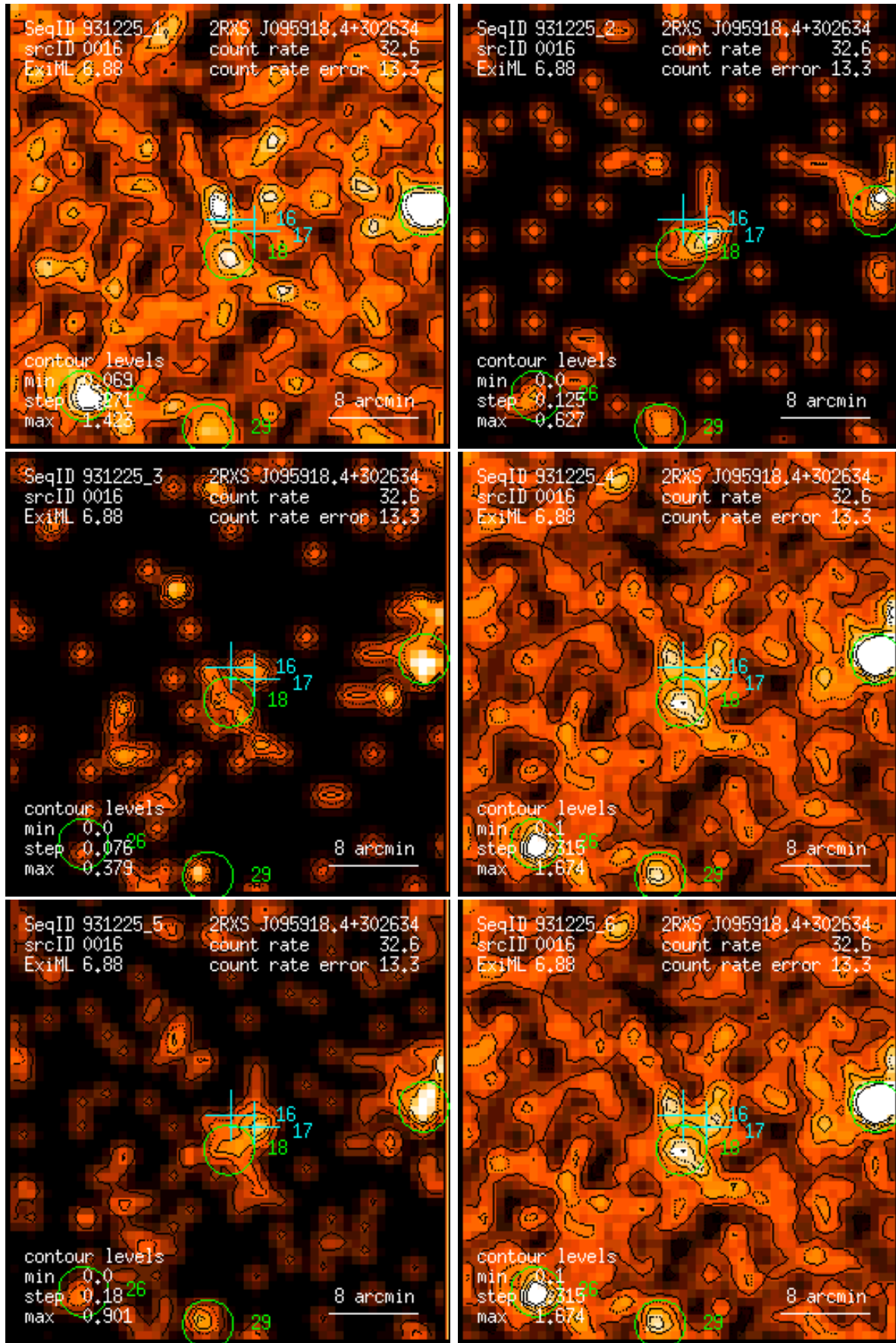
Figure 16: RASS 931225: detection 0016: band rate images, Gaussian filter: (1) PSPC channels 11 – 41, (2) 52 – 90, (3) 91 – 201, (4) 11 – 235, (5) 52 – 201, (6) 11 – 201. Broad band rates in counts/ks. Band rate contour levels in counts/ks/arcmin 2 .
