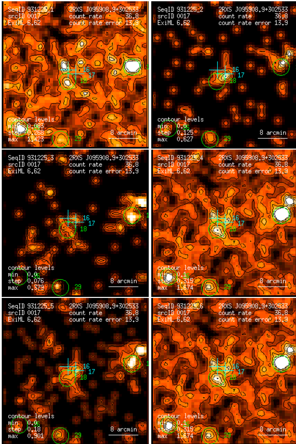
Figure 17: RASS 931225: detection 0017: band rate images, Gaussian filter: (1) PSPC channels 11 – 41, (2) 52 – 90, (3) 91 – 201, (4) 11 – 235, (5) 52 – 201, (6) 11 – 201. Broad band rates in counts/ks. Band rate contour levels in counts/ks/arcmin 2 .
