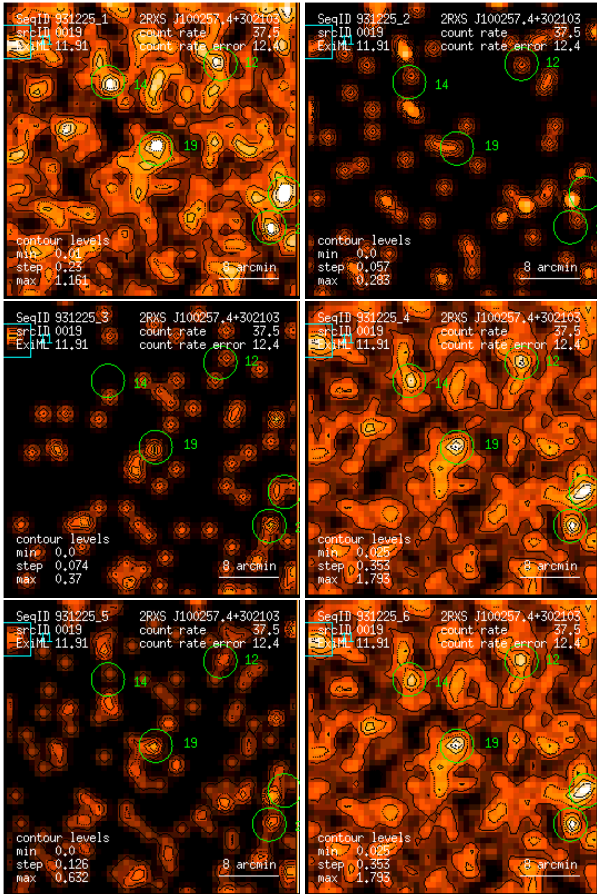
Figure 19: RASS 931225: detection 0019: band rate images, Gaussian filter: (1) PSPC channels 11 – 41, (2) 52 – 90, (3) 91 – 201, (4) 11 – 235, (5) 52 – 201, (6) 11 – 201. Broad band rates in counts/ks. Band rate contour levels in counts/ks/arcmin 2 .
