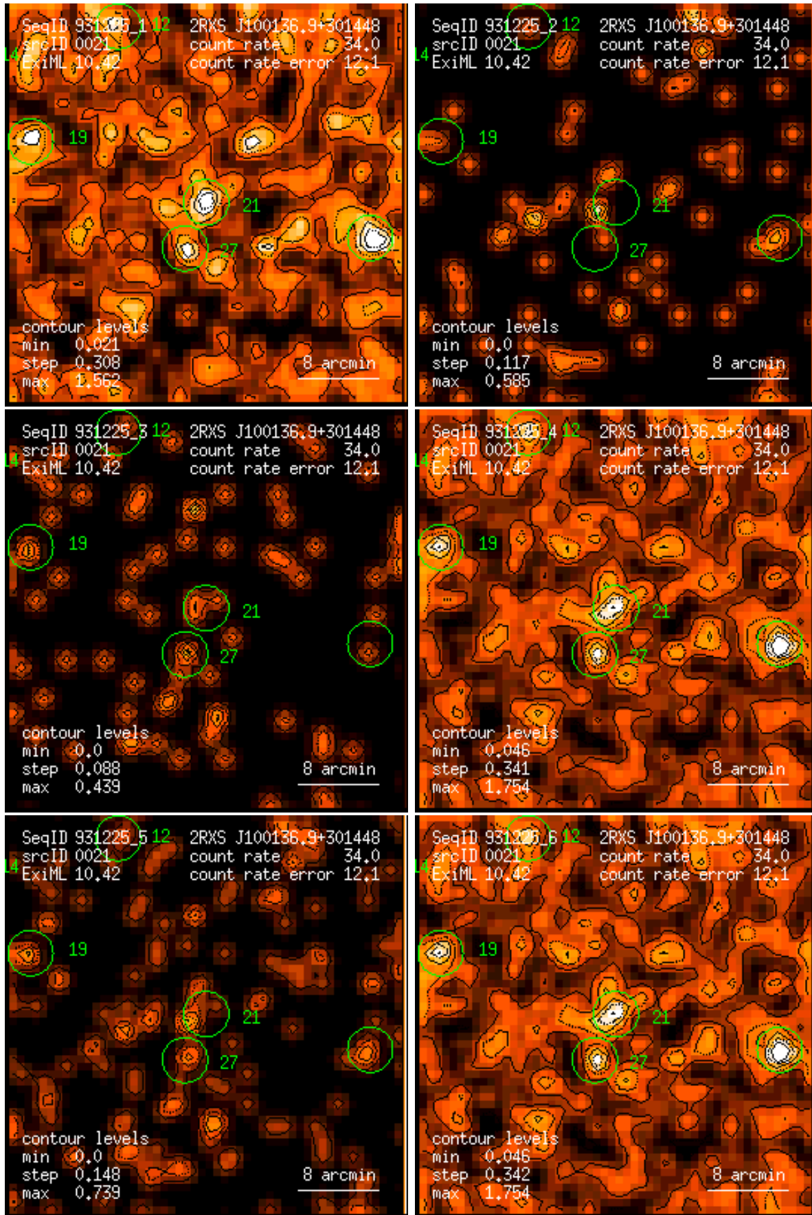
Figure 21: RASS 931225: detection 0021: band rate images, Gaussian filter: (1) PSPC channels 11 – 41, (2) 52 – 90, (3) 91 – 201, (4) 11 – 235, (5) 52 – 201, (6) 11 – 201. Broad band rates in counts/ks. Band rate contour levels in counts/ks/arcmin 2 .
