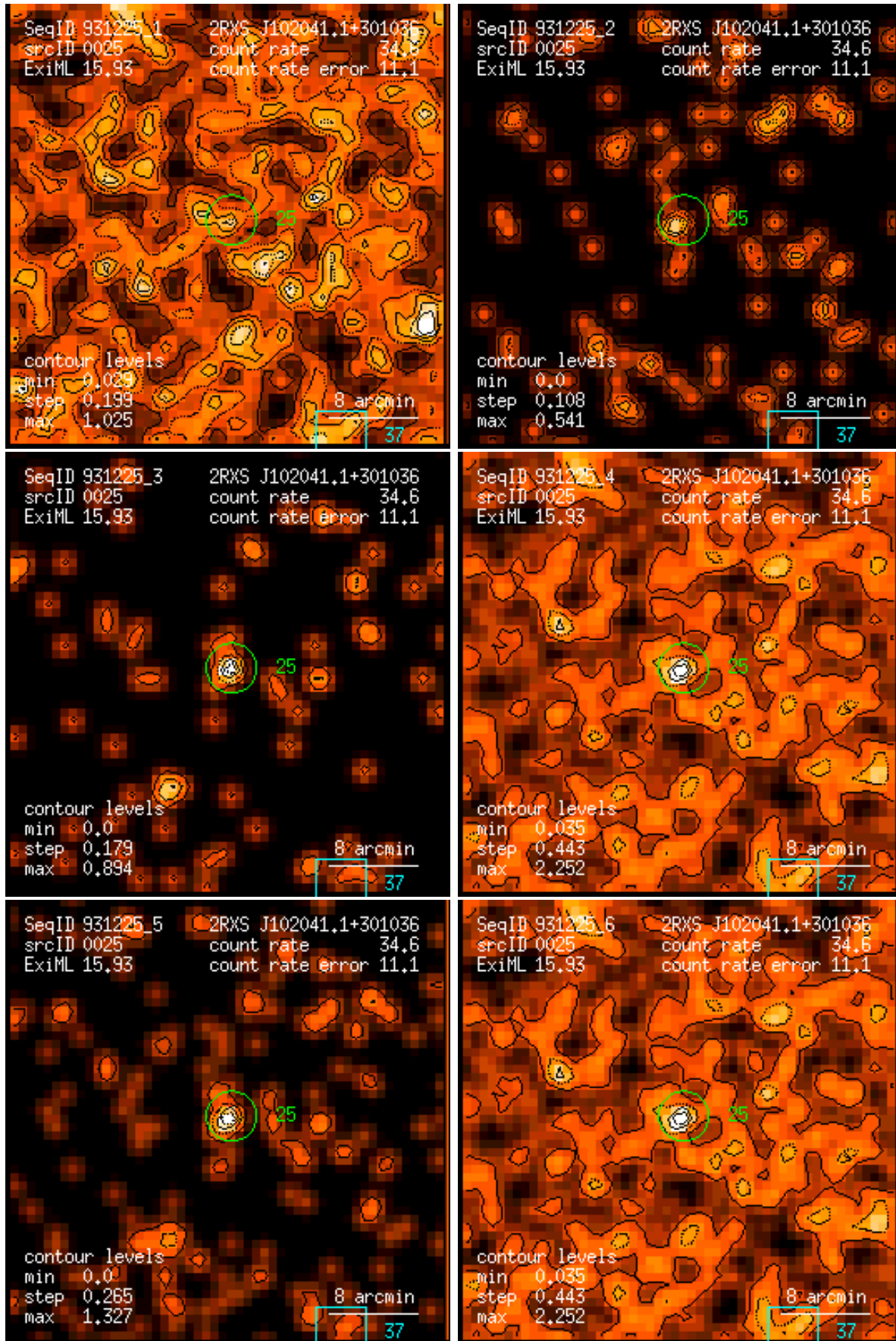
Figure 25: RASS 931225: detection 0025: band rate images, Gaussian filter: (1) PSPC channels 11 – 41, (2) 52 – 90, (3) 91 – 201, (4) 11 – 235, (5) 52 – 201, (6) 11 – 201. Broad band rates in counts/ks. Band rate contour levels in counts/ks/arcmin 2 .
