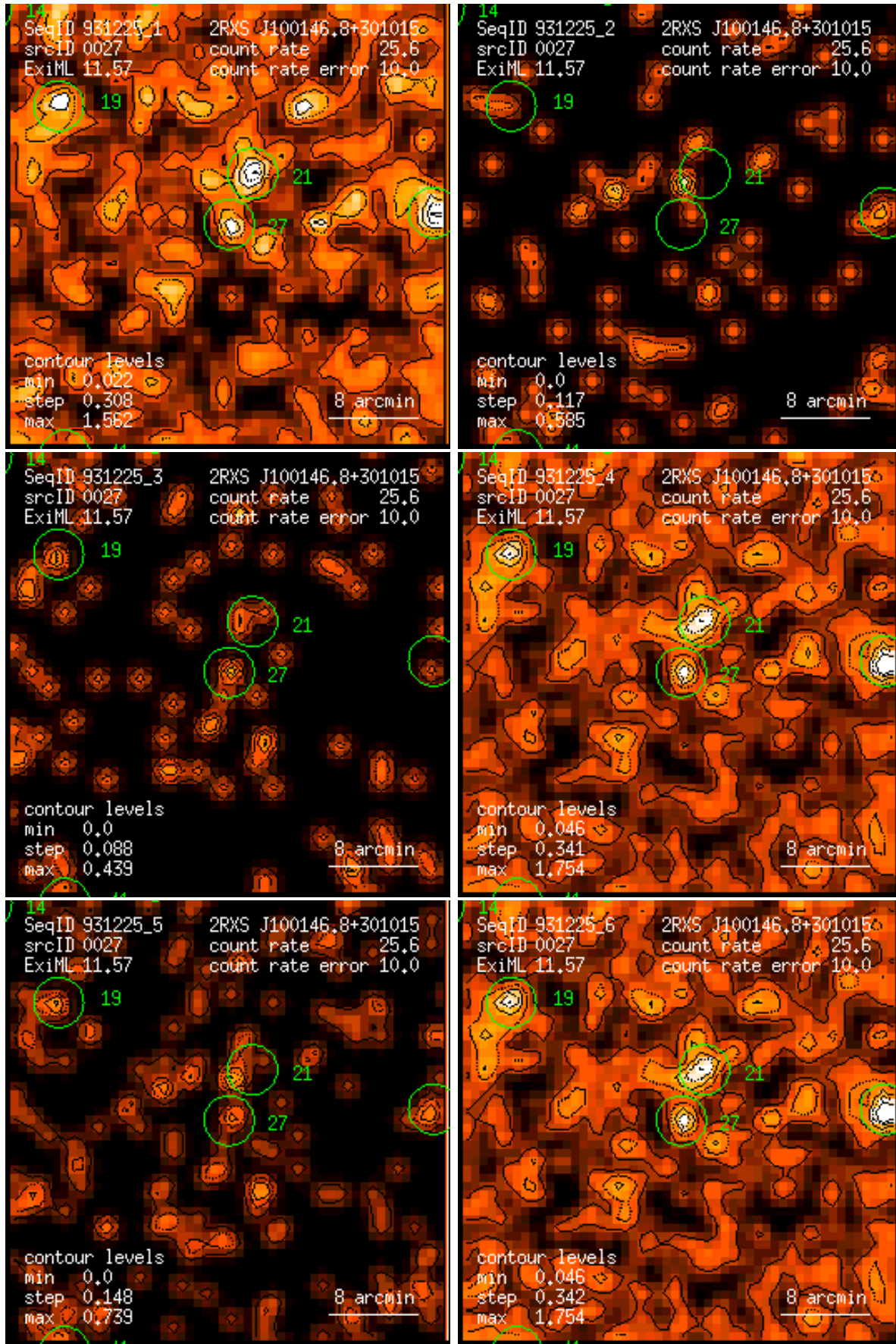
Figure 27: RASS 931225: detection 0027: band rate images, Gaussian filter: (1) PSPC channels 11 – 41, (2) 52 – 90, (3) 91 – 201, (4) 11 – 235, (5) 52 – 201, (6) 11 – 201. Broad band rates in counts/ks. Band rate contour levels in counts/ks/arcmin 2 .
