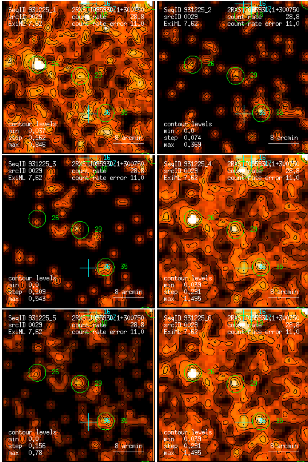
Figure 29: RASS 931225: detection 0029: band rate images, Gaussian filter: (1) PSPC channels 11 – 41, (2) 52 – 90, (3) 91 – 201, (4) 11 – 235, (5) 52 – 201, (6) 11 – 201. Broad band rates in counts/ks. Band rate contour levels in counts/ks/arcmin 2 .
