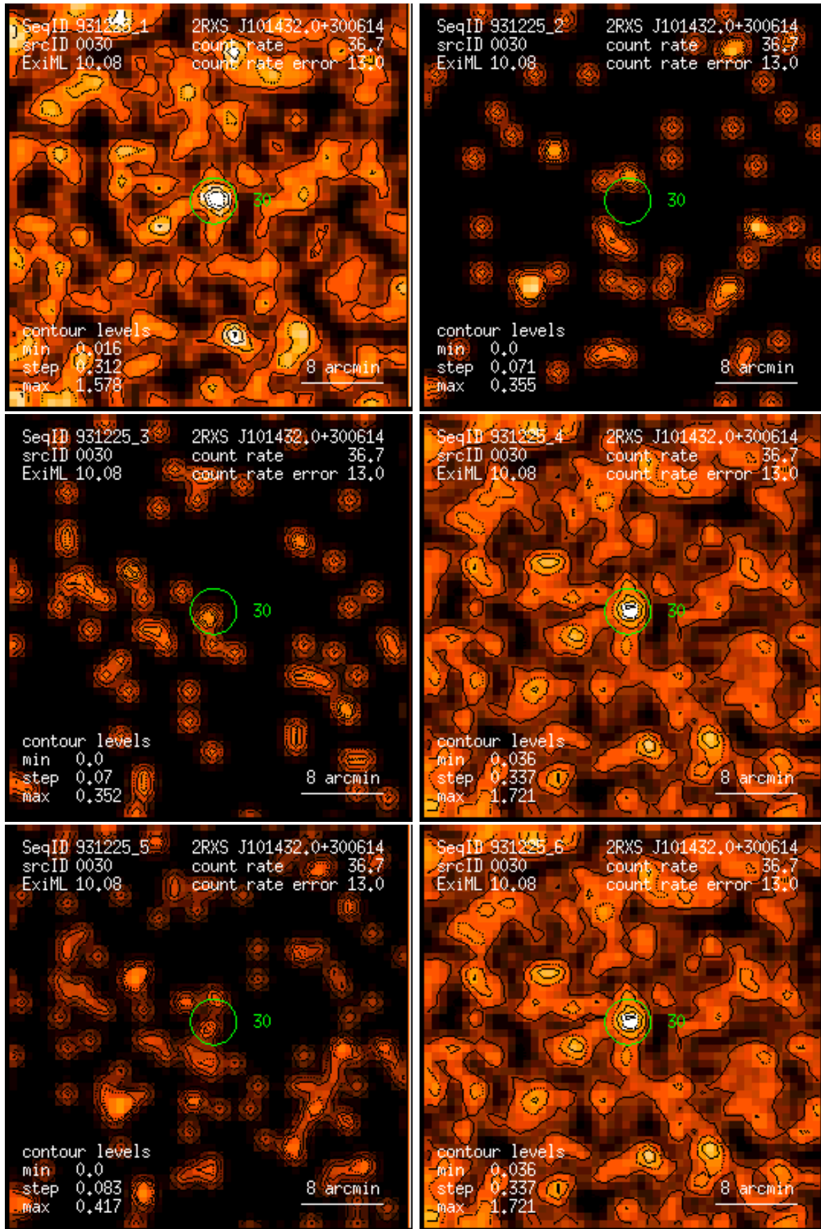
Figure 30: RASS 931225: detection 0030: band rate images, Gaussian filter: (1) PSPC channels 11 – 41, (2) 52 – 90, (3) 91 – 201, (4) 11 – 235, (5) 52 – 201, (6) 11 – 201. Broad band rates in counts/ks. Band rate contour levels in counts/ks/arcmin 2 .
