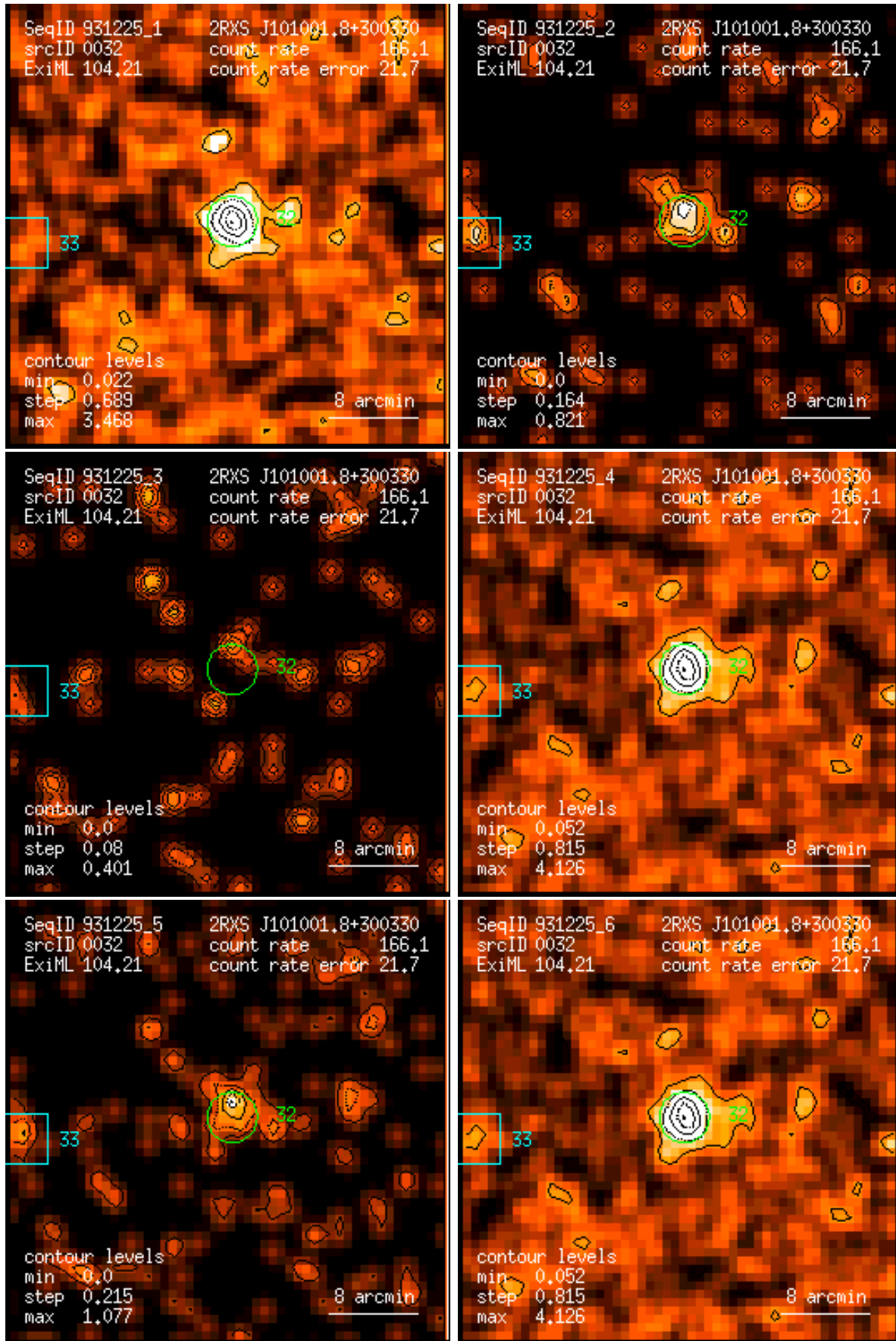
Figure 32: RASS 931225: detection 0032: band rate images, Gaussian filter: (1) PSPC channels 11 – 41, (2) 52 – 90, (3) 91 – 201, (4) 11 – 235, (5) 52 – 201, (6) 11 – 201. Broad band rates in counts/ks. Band rate contour levels in counts/ks/arcmin 2 .
