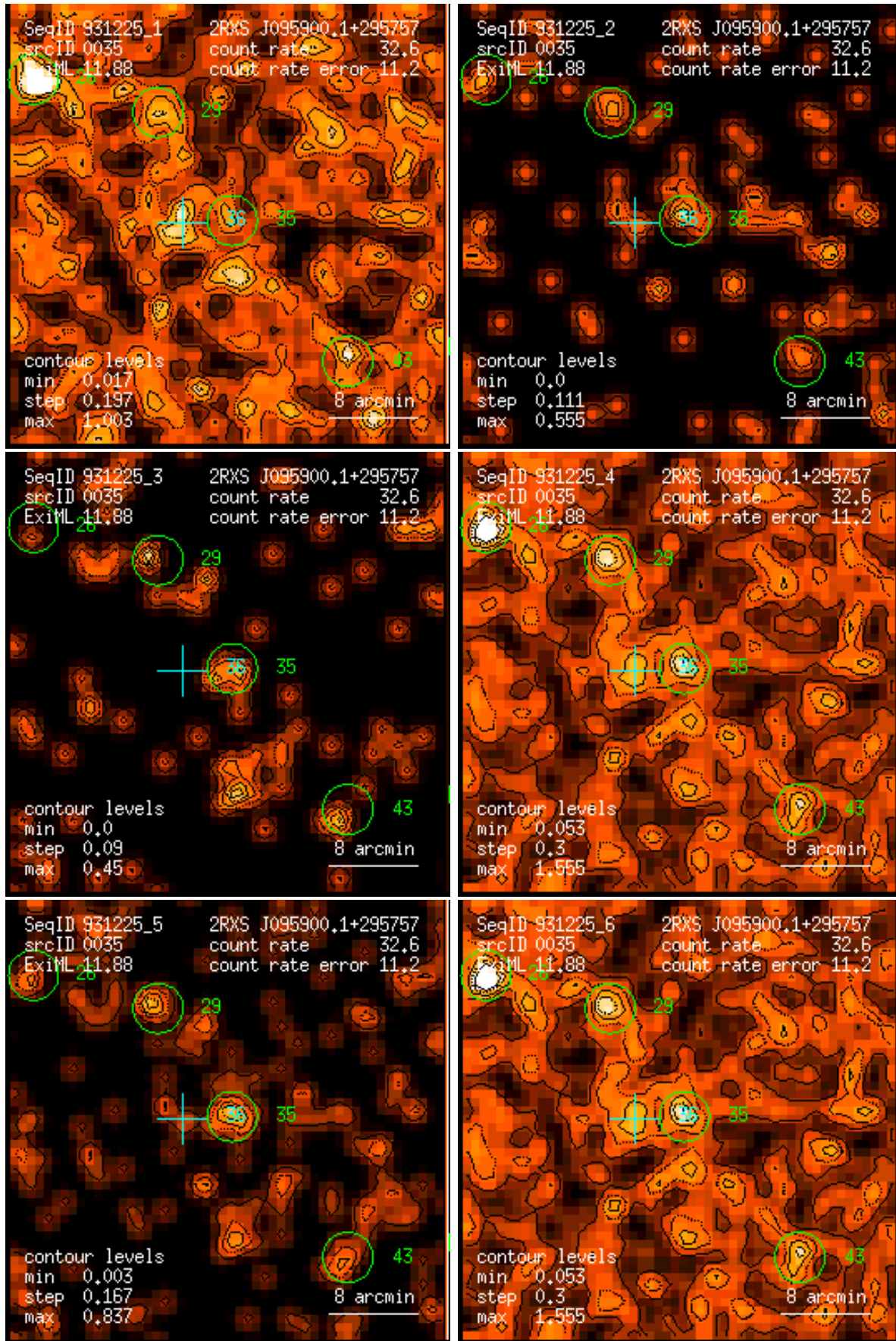
Figure 35: RASS 931225: detection 0035: band rate images, Gaussian filter: (1) PSPC channels 11 – 41, (2) 52 – 90, (3) 91 – 201, (4) 11 – 235, (5) 52 – 201, (6) 11 – 201. Broad band rates in counts/ks. Band rate contour levels in counts/ks/arcmin 2 .
