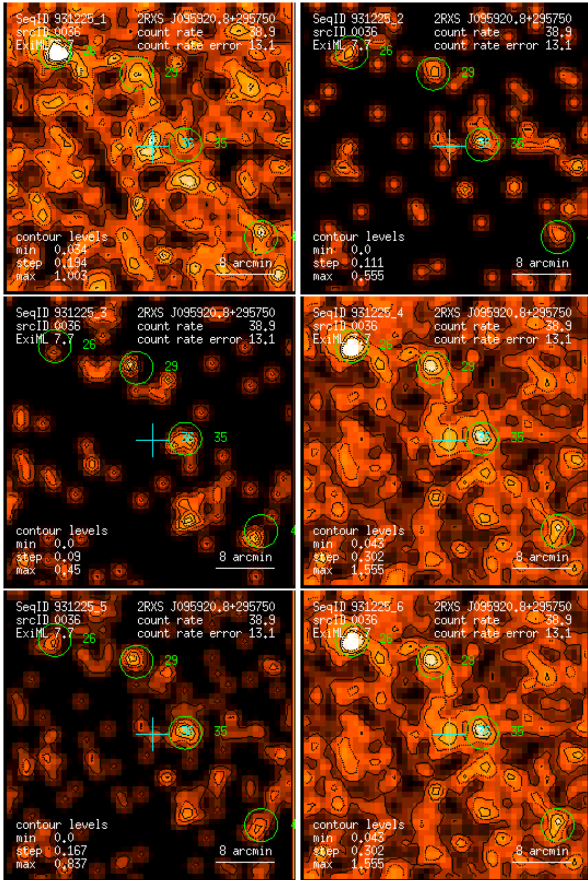
Figure 36: RASS 931225: detection 0036: band rate images, Gaussian filter: (1) PSPC channels 11 – 41, (2) 52 – 90, (3) 91 – 201, (4) 11 – 235, (5) 52 – 201, (6) 11 – 201. Broad band rates in counts/ks. Band rate contour levels in counts/ks/arcmin 2 .
