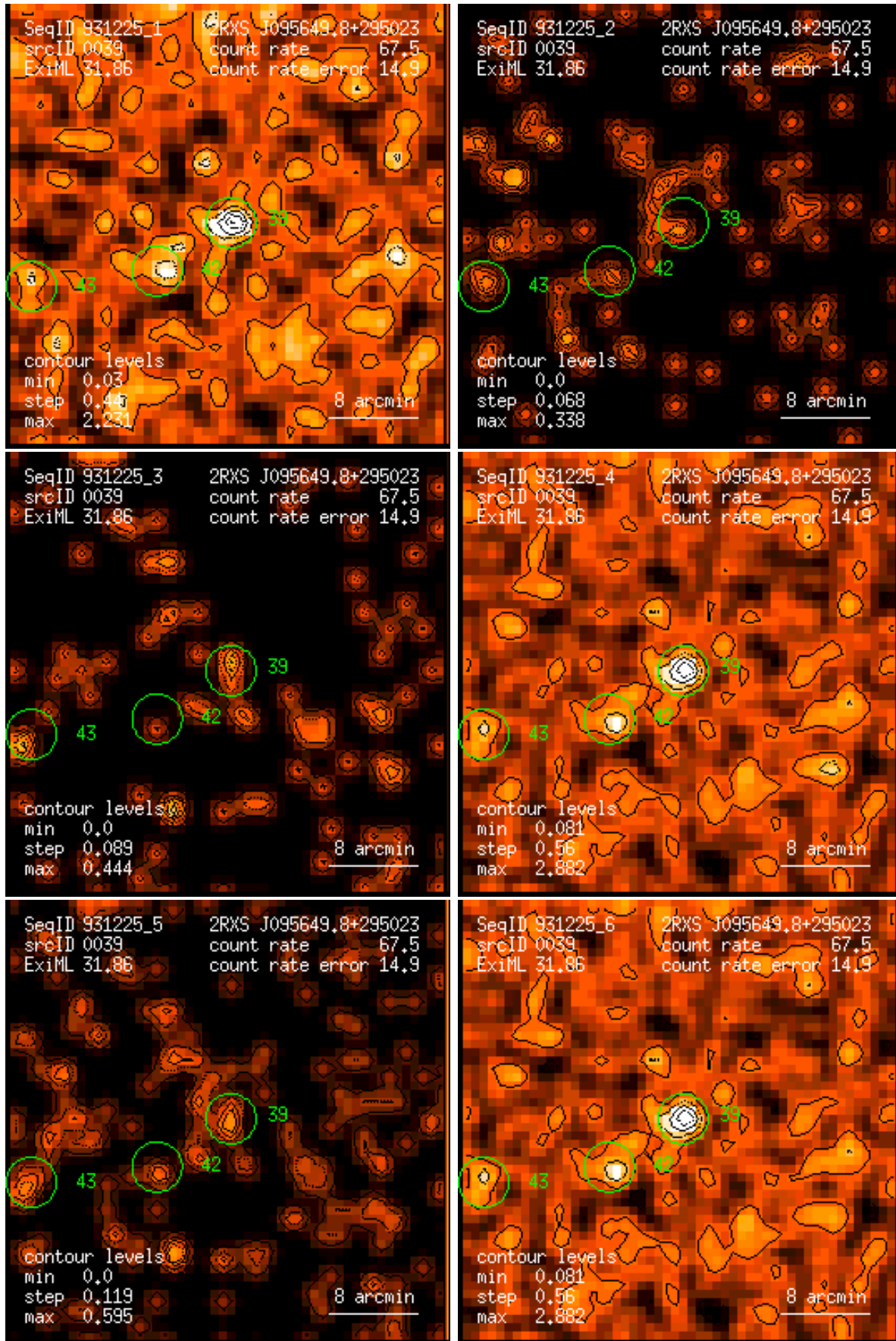
Figure 39: RASS 931225: detection 0039: band rate images, Gaussian filter: (1) PSPC channels 11 – 41, (2) 52 – 90, (3) 91 – 201, (4) 11 – 235, (5) 52 – 201, (6) 11 – 201. Broad band rates in counts/ks. Band rate contour levels in counts/ks/arcmin 2 .
