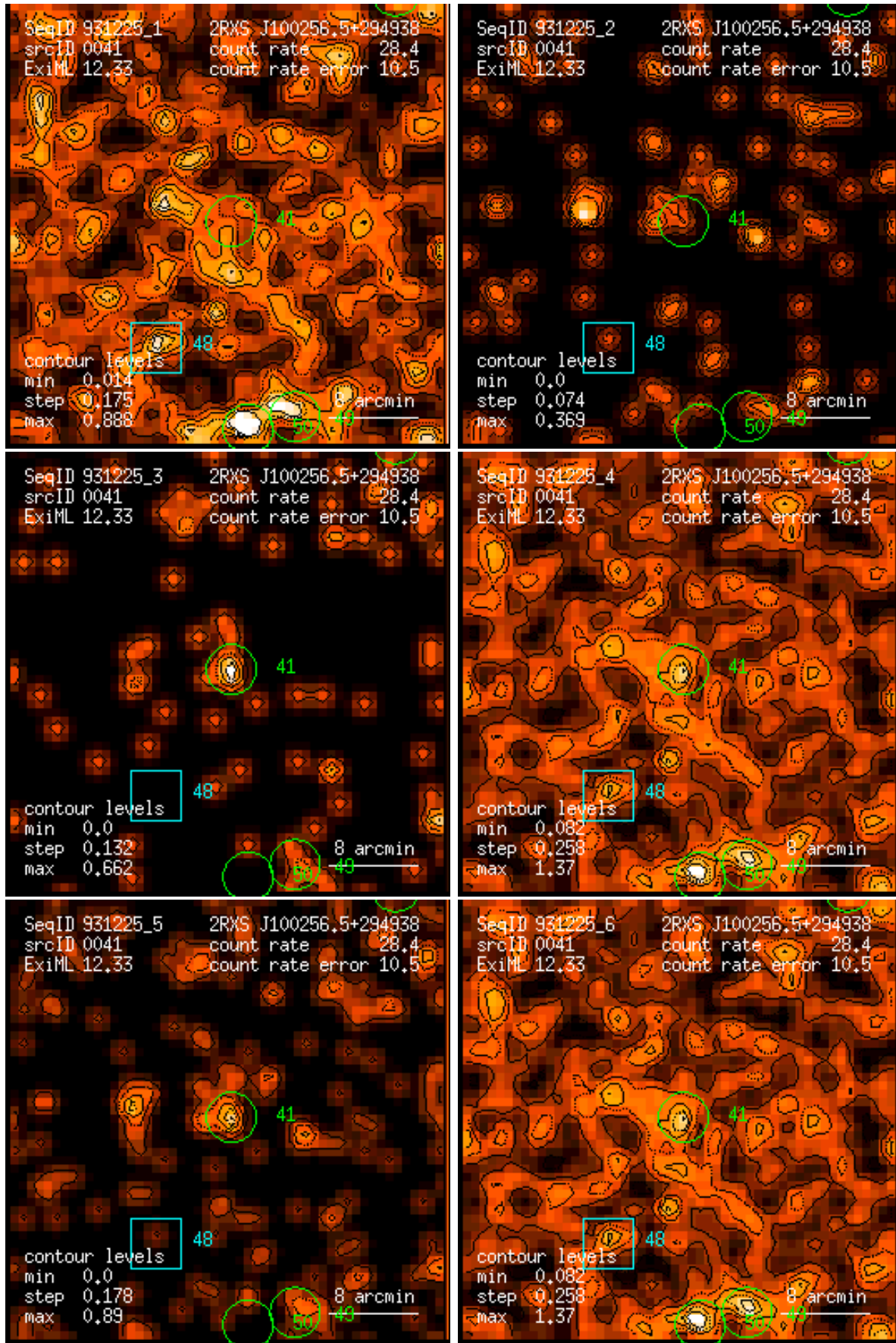
Figure 41: RASS 931225: detection 0041: band rate images, Gaussian filter: (1) PSPC channels 11 – 41, (2) 52 – 90, (3) 91 – 201, (4) 11 – 235, (5) 52 – 201, (6) 11 – 201. Broad band rates in counts/ks. Band rate contour levels in counts/ks/arcmin 2 .
