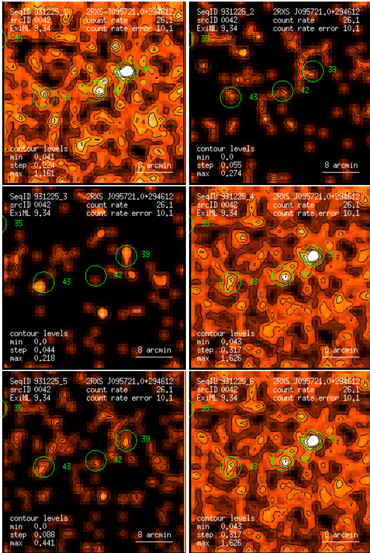
Figure 42: RASS 931225: detection 0042: band rate images, Gaussian filter: (1) PSPC channels 11 – 41, (2) 52 – 90, (3) 91 – 201, (4) 11 – 235, (5) 52 – 201, (6) 11 – 201. Broad band rates in counts/ks. Band rate contour levels in counts/ks/arcmin 2 .
