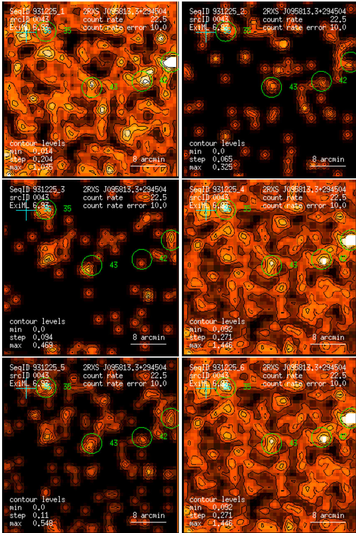
Figure 43: RASS 931225: detection 0043: band rate images, Gaussian filter: (1) PSPC channels 11 – 41, (2) 52 – 90, (3) 91 – 201, (4) 11 – 235, (5) 52 – 201, (6) 11 – 201. Broad band rates in counts/ks. Band rate contour levels in counts/ks/arcmin 2 .
