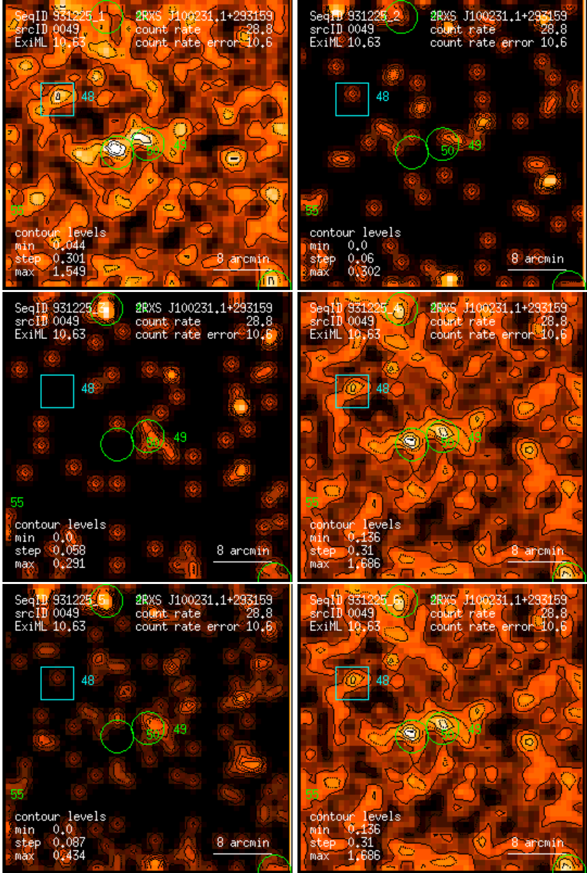
Figure 49: RASS 931225: detection 0049: band rate images, Gaussian filter: (1) PSPC channels 11 – 41, (2) 52 – 90, (3) 91 – 201, (4) 11 – 235, (5) 52 – 201, (6) 11 – 201. Broad band rates in counts/ks. Band rate contour levels in counts/ks/arcmin 2 .
