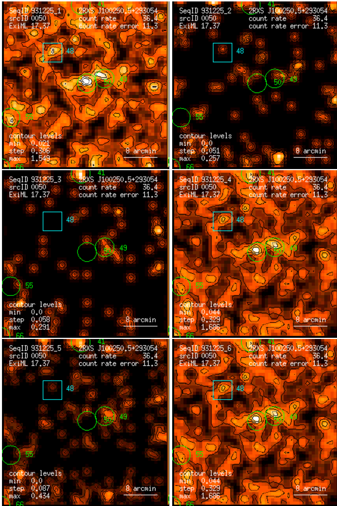
Figure 50: RASS 931225: detection 0050: band rate images, Gaussian filter: (1) PSPC channels 11 – 41, (2) 52 – 90, (3) 91 – 201, (4) 11 – 235, (5) 52 – 201, (6) 11 – 201. Broad band rates in counts/ks. Band rate contour levels in counts/ks/arcmin 2 .
