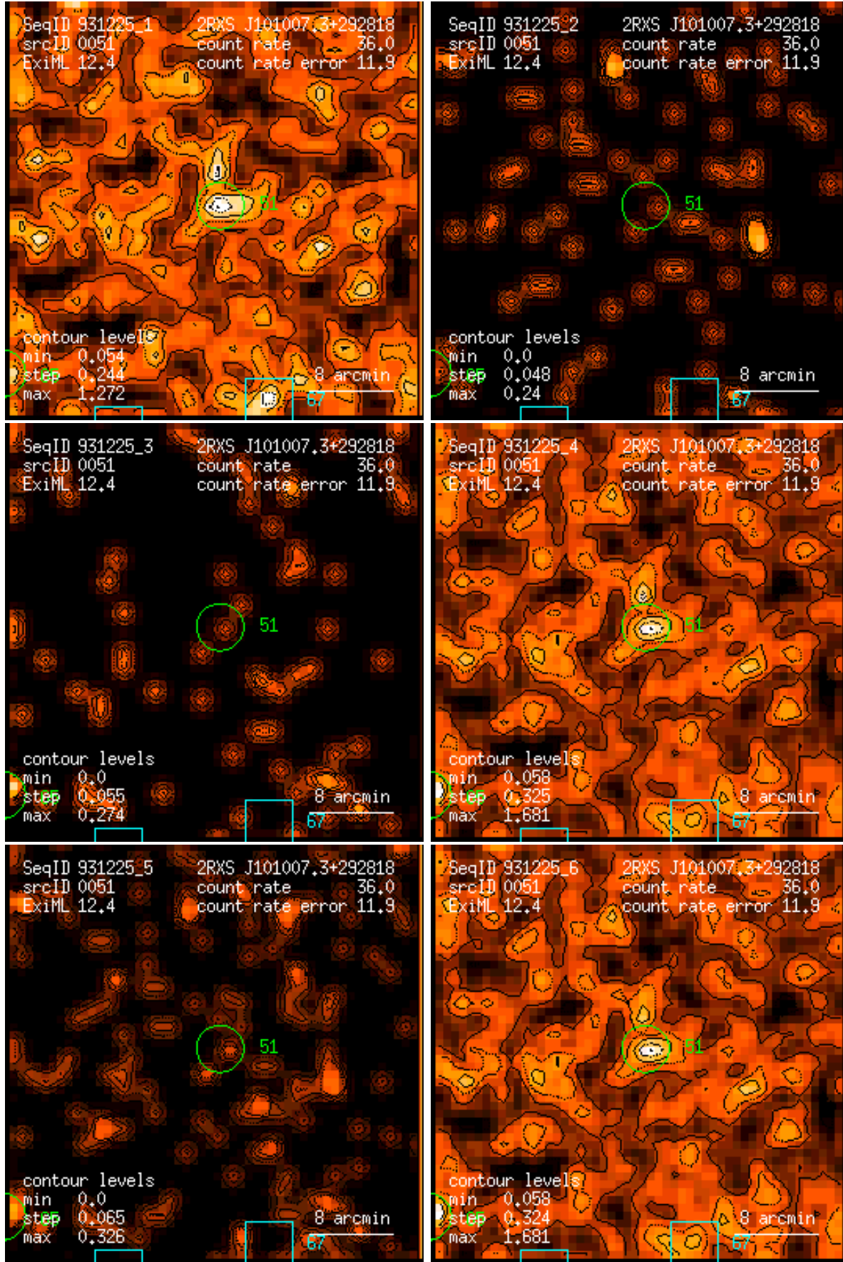
Figure 51: RASS 931225: detection 0051: band rate images, Gaussian filter: (1) PSPC channels 11 – 41, (2) 52 – 90, (3) 91 – 201, (4) 11 – 235, (5) 52 – 201, (6) 11 – 201. Broad band rates in counts/ks. Band rate contour levels in counts/ks/arcmin 2 .
