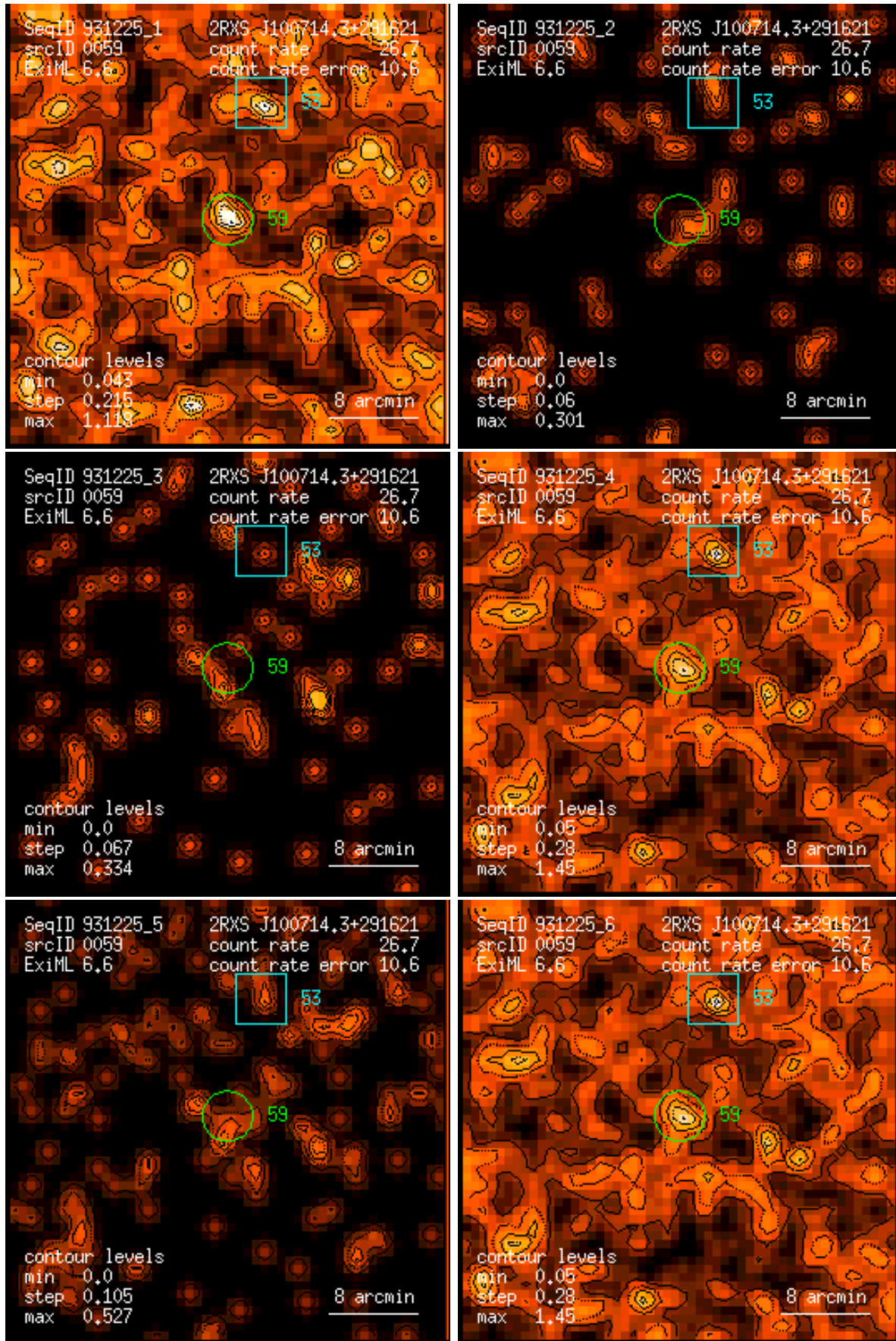
Figure 59: RASS 931225: detection 0059: band rate images, Gaussian filter: (1) PSPC channels 11 – 41, (2) 52 – 90, (3) 91 – 201, (4) 11 – 235, (5) 52 – 201, (6) 11 – 201. Broad band rates in counts/ks. Band rate contour levels in counts/ks/arcmin 2 .
