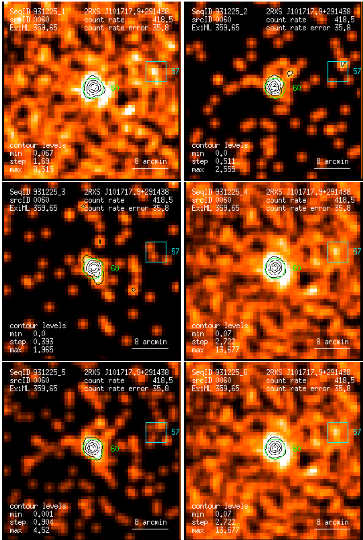
Figure 60: RASS 931225: detection 0060: band rate images, Gaussian filter: (1) PSPC channels 11 – 41, (2) 52 – 90, (3) 91 – 201, (4) 11 – 235, (5) 52 – 201, (6) 11 – 201. Broad band rates in counts/ks. Band rate contour levels in counts/ks/arcmin 2 .
