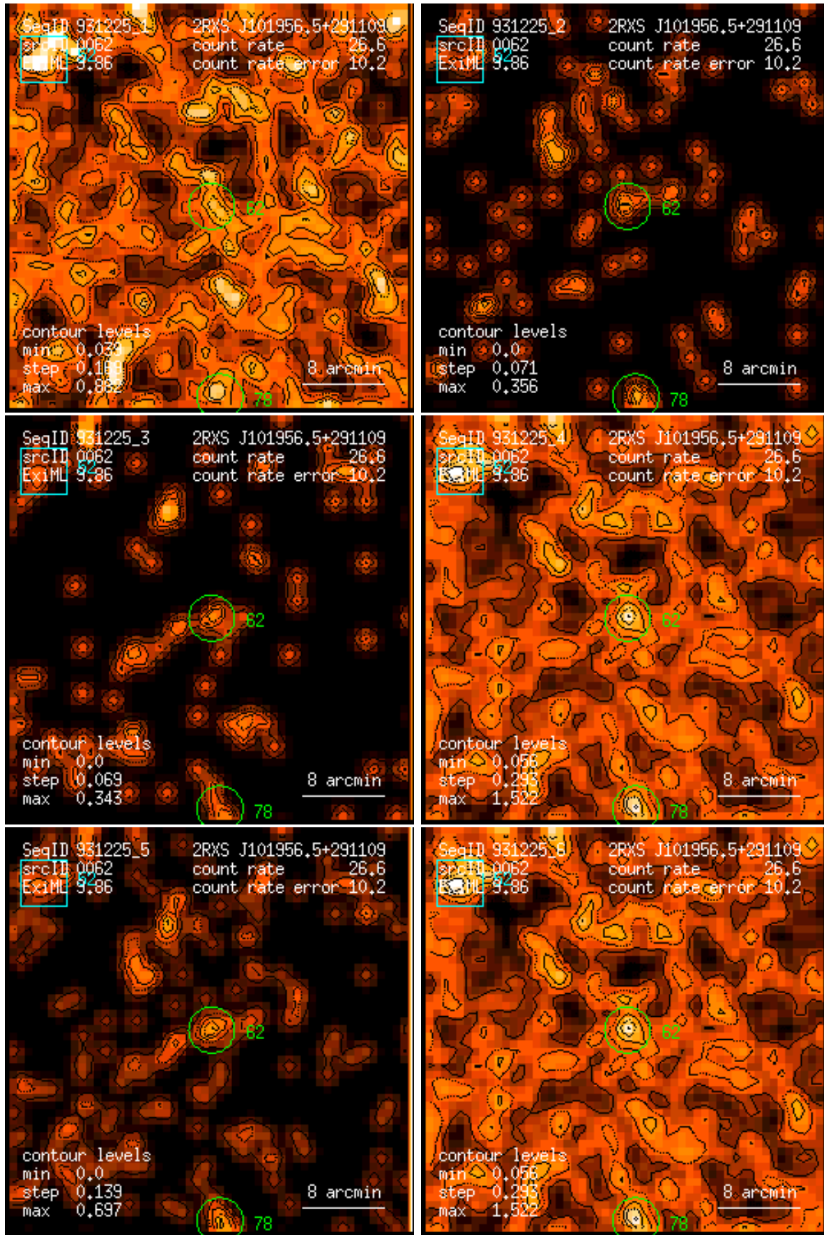
Figure 62: RASS 931225: detection 0062: band rate images, Gaussian filter: (1) PSPC channels 11 – 41, (2) 52 – 90, (3) 91 – 201, (4) 11 – 235, (5) 52 – 201, (6) 11 – 201. Broad band rates in counts/ks. Band rate contour levels in counts/ks/arcmin 2 .
