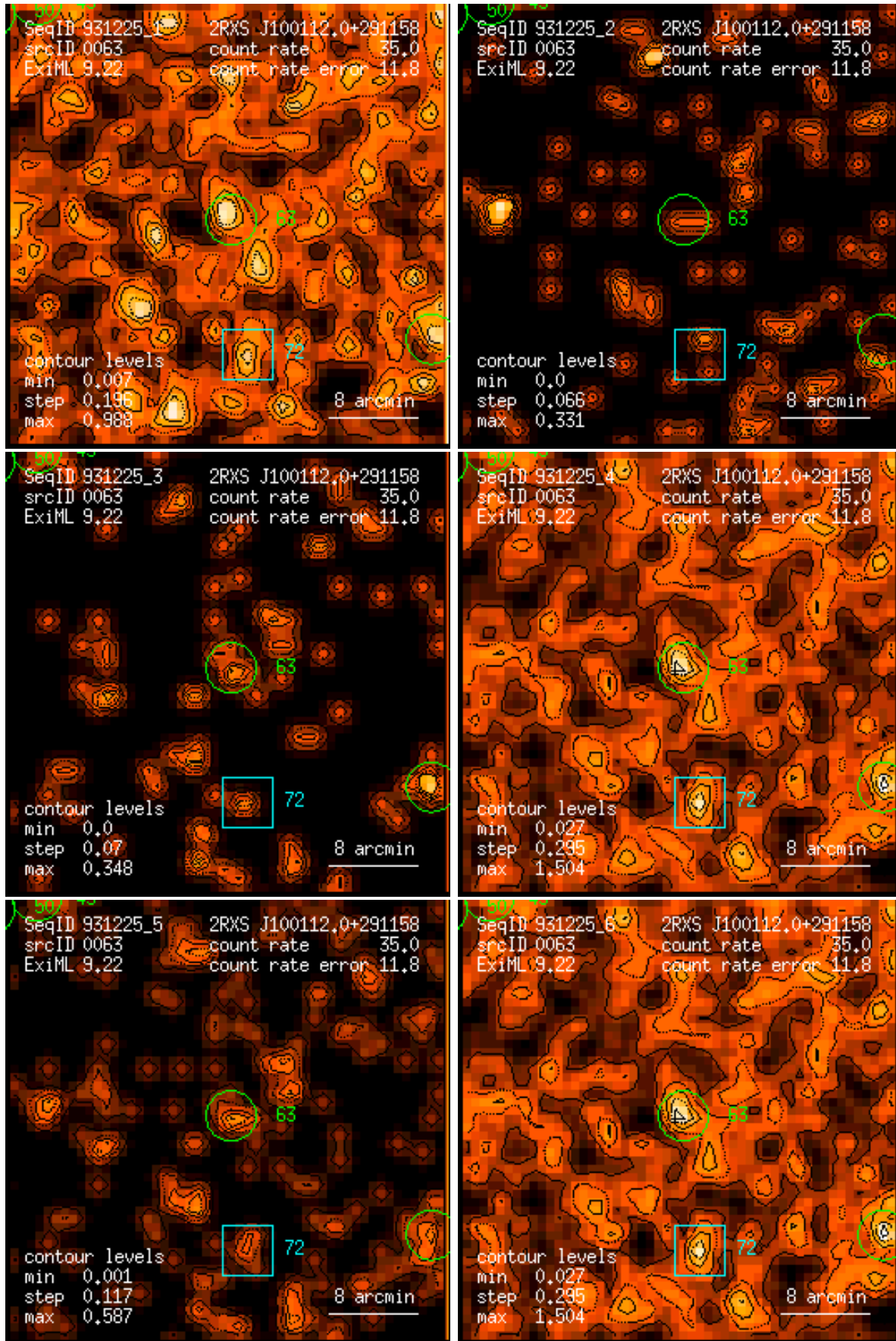
Figure 63: RASS 931225: detection 0063: band rate images, Gaussian filter: (1) PSPC channels 11 – 41, (2) 52 – 90, (3) 91 – 201, (4) 11 – 235, (5) 52 – 201, (6) 11 – 201. Broad band rates in counts/ks. Band rate contour levels in counts/ks/arcmin 2 .
