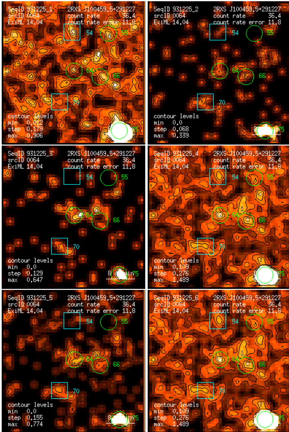
Figure 64: RASS 931225: detection 0064: band rate images, Gaussian filter: (1) PSPC channels 11 – 41, (2) 52 – 90, (3) 91 – 201, (4) 11 – 235, (5) 52 – 201, (6) 11 – 201. Broad band rates in counts/ks. Band rate contour levels in counts/ks/arcmin 2 .
