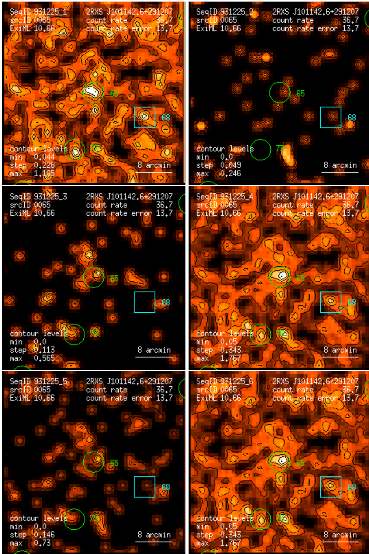
Figure 65: RASS 931225: detection 0065: band rate images, Gaussian filter: (1) PSPC channels 11 – 41, (2) 52 – 90, (3) 91 – 201, (4) 11 – 235, (5) 52 – 201, (6) 11 – 201. Broad band rates in counts/ks. Band rate contour levels in counts/ks/arcmin 2 .
