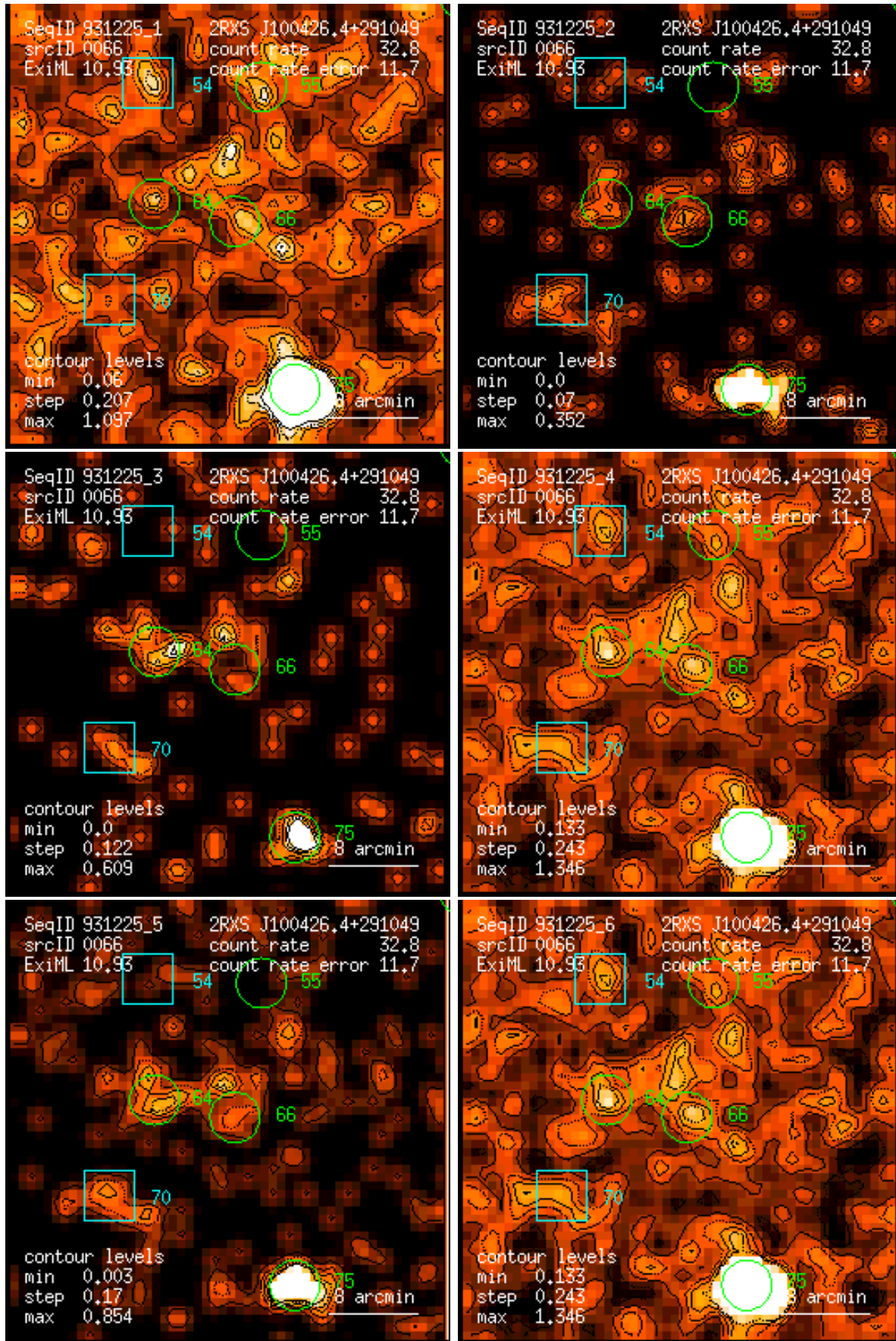
Figure 66: RASS 931225: detection 0066: band rate images, Gaussian filter: (1) PSPC channels 11 – 41, (2) 52 – 90, (3) 91 – 201, (4) 11 – 235, (5) 52 – 201, (6) 11 – 201. Broad band rates in counts/ks. Band rate contour levels in counts/ks/arcmin 2 .
