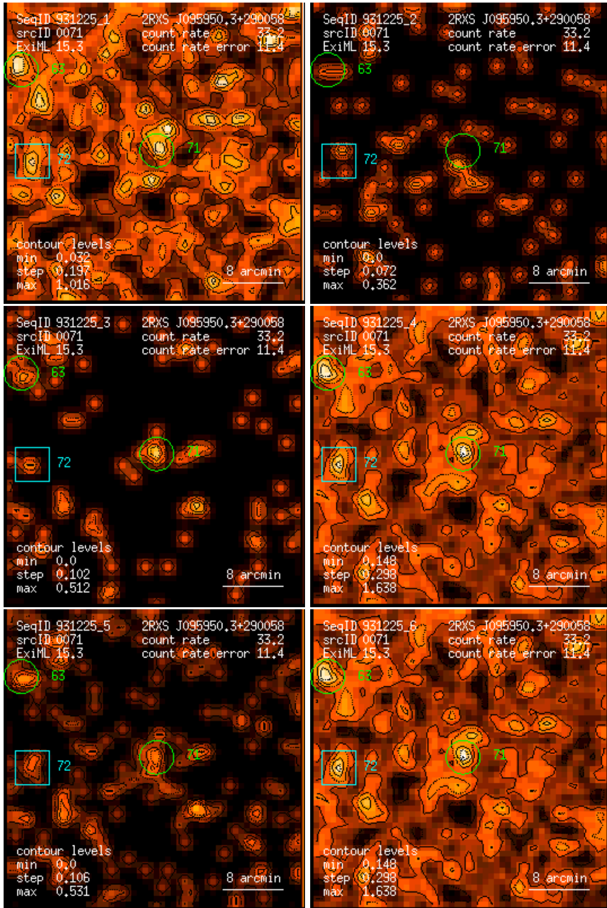
Figure 71: RASS 931225: detection 0071: band rate images, Gaussian filter: (1) PSPC channels 11 – 41, (2) 52 – 90, (3) 91 – 201, (4) 11 – 235, (5) 52 – 201, (6) 11 – 201. Broad band rates in counts/ks. Band rate contour levels in counts/ks/arcmin 2 .
