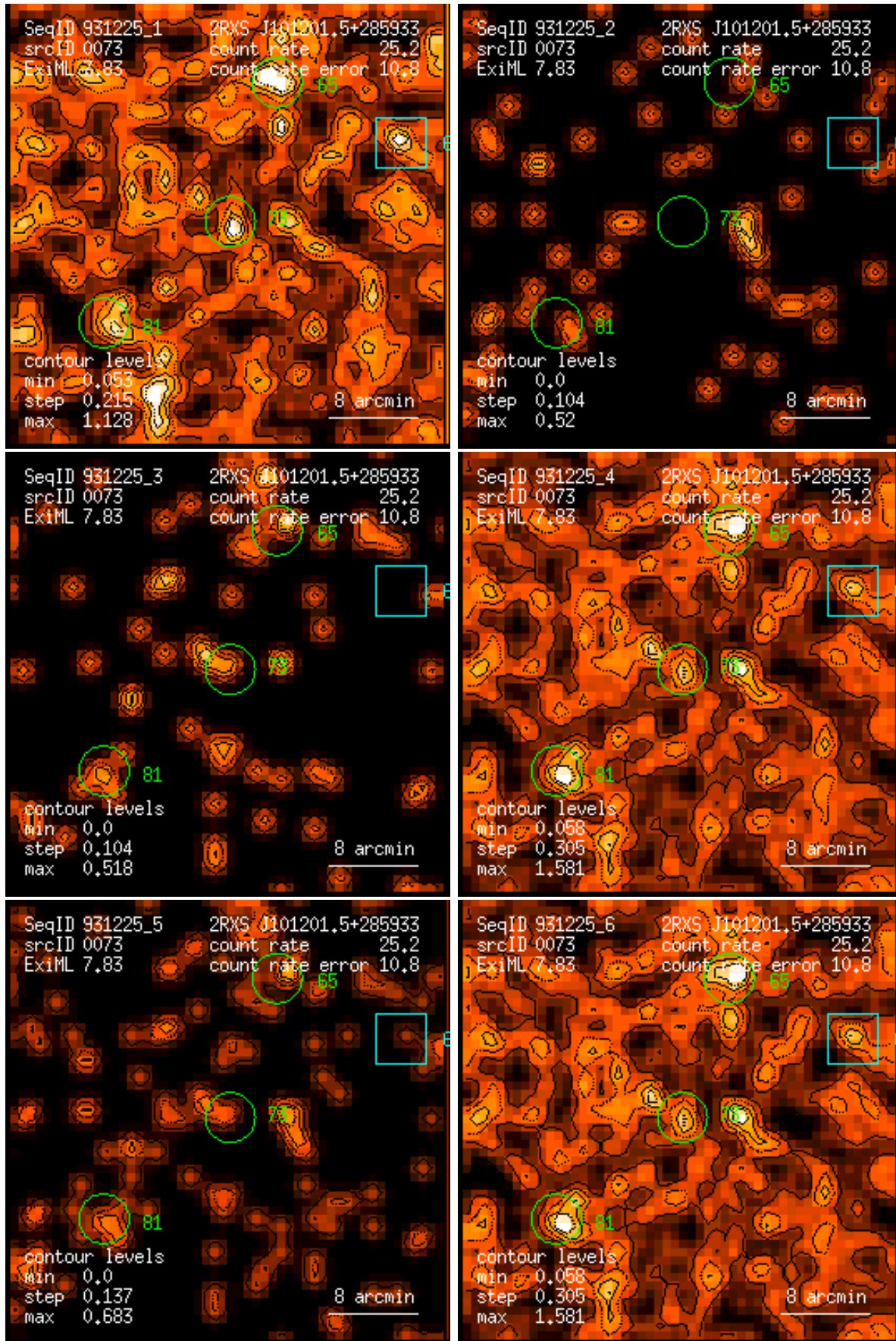
Figure 73: RASS 931225: detection 0073: band rate images, Gaussian filter: (1) PSPC channels 11 – 41, (2) 52 – 90, (3) 91 – 201, (4) 11 – 235, (5) 52 – 201, (6) 11 – 201. Broad band rates in counts/ks. Band rate contour levels in counts/ks/arcmin 2 .
