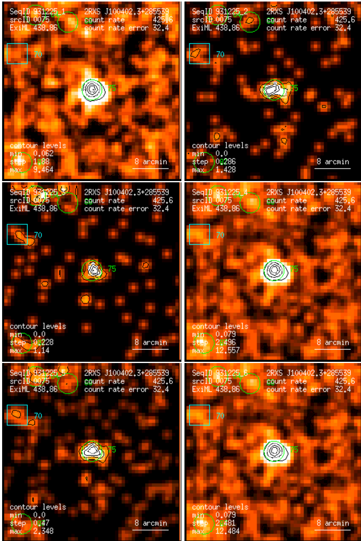
Figure 75: RASS 931225: detection 0075: band rate images, Gaussian filter: (1) PSPC channels 11 – 41, (2) 52 – 90, (3) 91 – 201, (4) 11 – 235, (5) 52 – 201, (6) 11 – 201. Broad band rates in counts/ks. Band rate contour levels in counts/ks/arcmin 2 .
