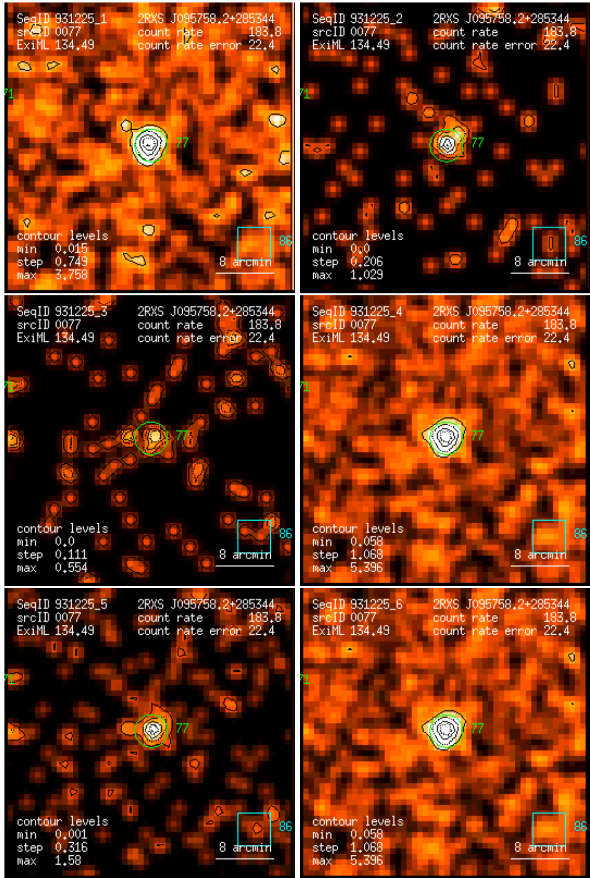
Figure 77: RASS 931225: detection 0077: band rate images, Gaussian filter: (1) PSPC channels 11 – 41, (2) 52 – 90, (3) 91 – 201, (4) 11 – 235, (5) 52 – 201, (6) 11 – 201. Broad band rates in counts/ks. Band rate contour levels in counts/ks/arcmin 2 .
