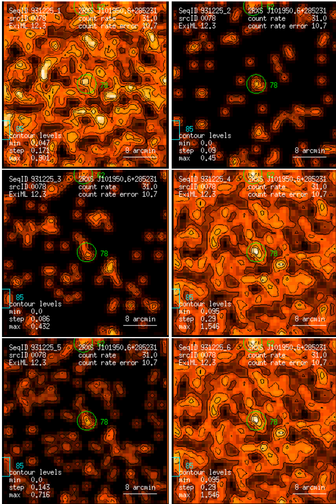
Figure 78: RASS 931225: detection 0078: band rate images, Gaussian filter: (1) PSPC channels 11 – 41, (2) 52 – 90, (3) 91 – 201, (4) 11 – 235, (5) 52 – 201, (6) 11 – 201. Broad band rates in counts/ks. Band rate contour levels in counts/ks/arcmin 2 .
