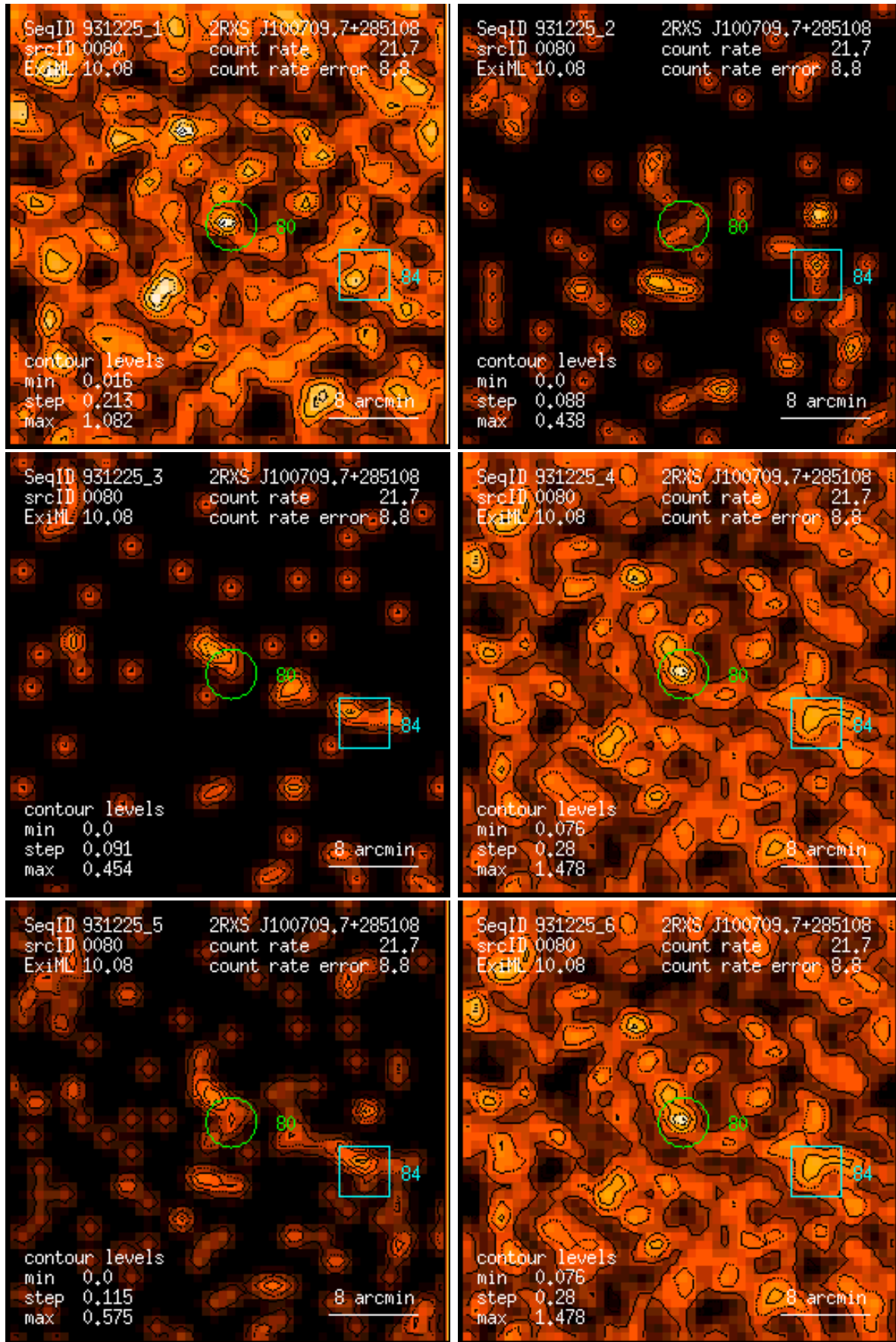
Figure 80: RASS 931225: detection 0080: band rate images, Gaussian filter: (1) PSPC channels 11 – 41, (2) 52 – 90, (3) 91 – 201, (4) 11 – 235, (5) 52 – 201, (6) 11 – 201. Broad band rates in counts/ks. Band rate contour levels in counts/ks/arcmin 2 .
