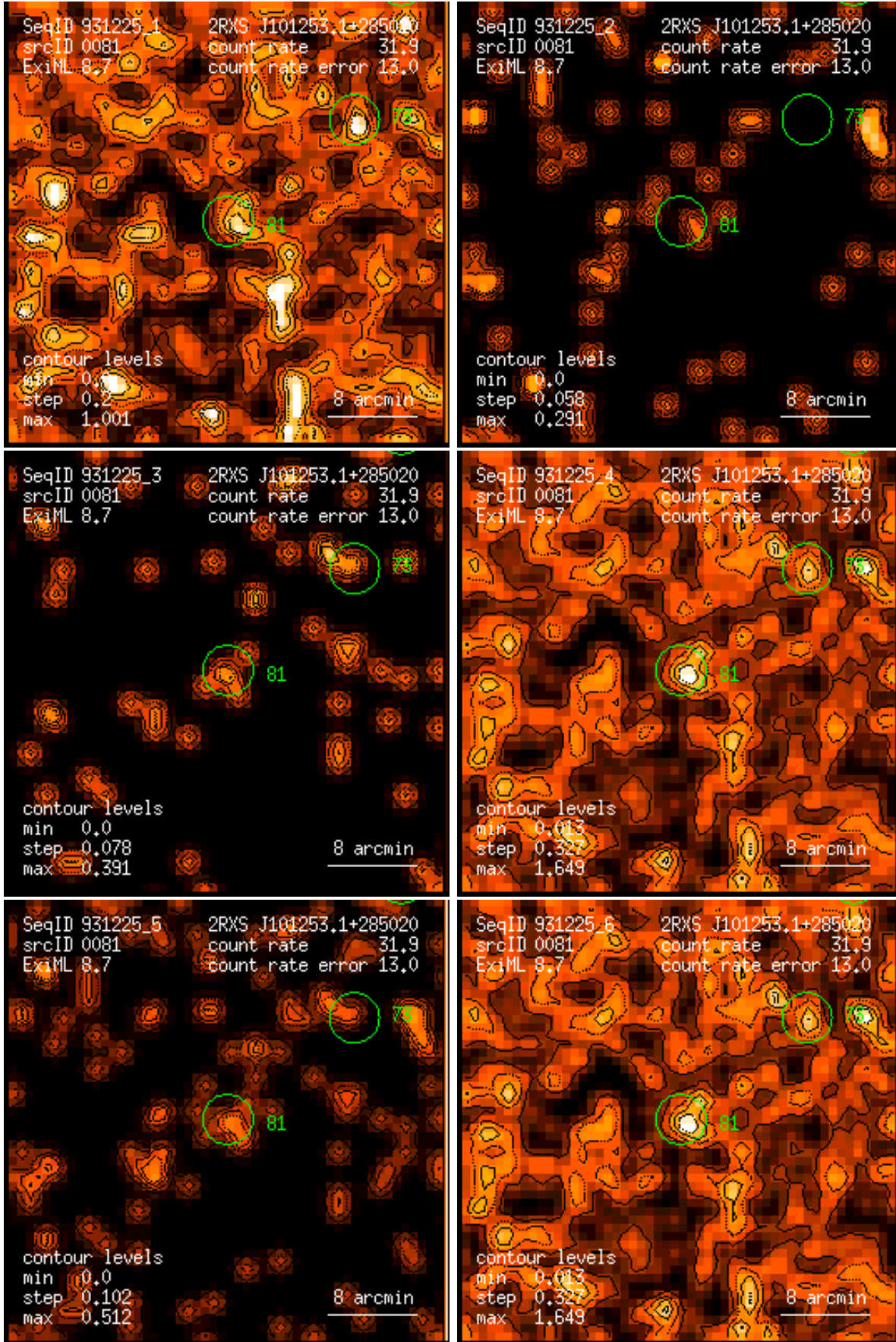
Figure 81: RASS 931225: detection 0081: band rate images, Gaussian filter: (1) PSPC channels 11 – 41, (2) 52 – 90, (3) 91 – 201, (4) 11 – 235, (5) 52 – 201, (6) 11 – 201. Broad band rates in counts/ks. Band rate contour levels in counts/ks/arcmin 2 .
