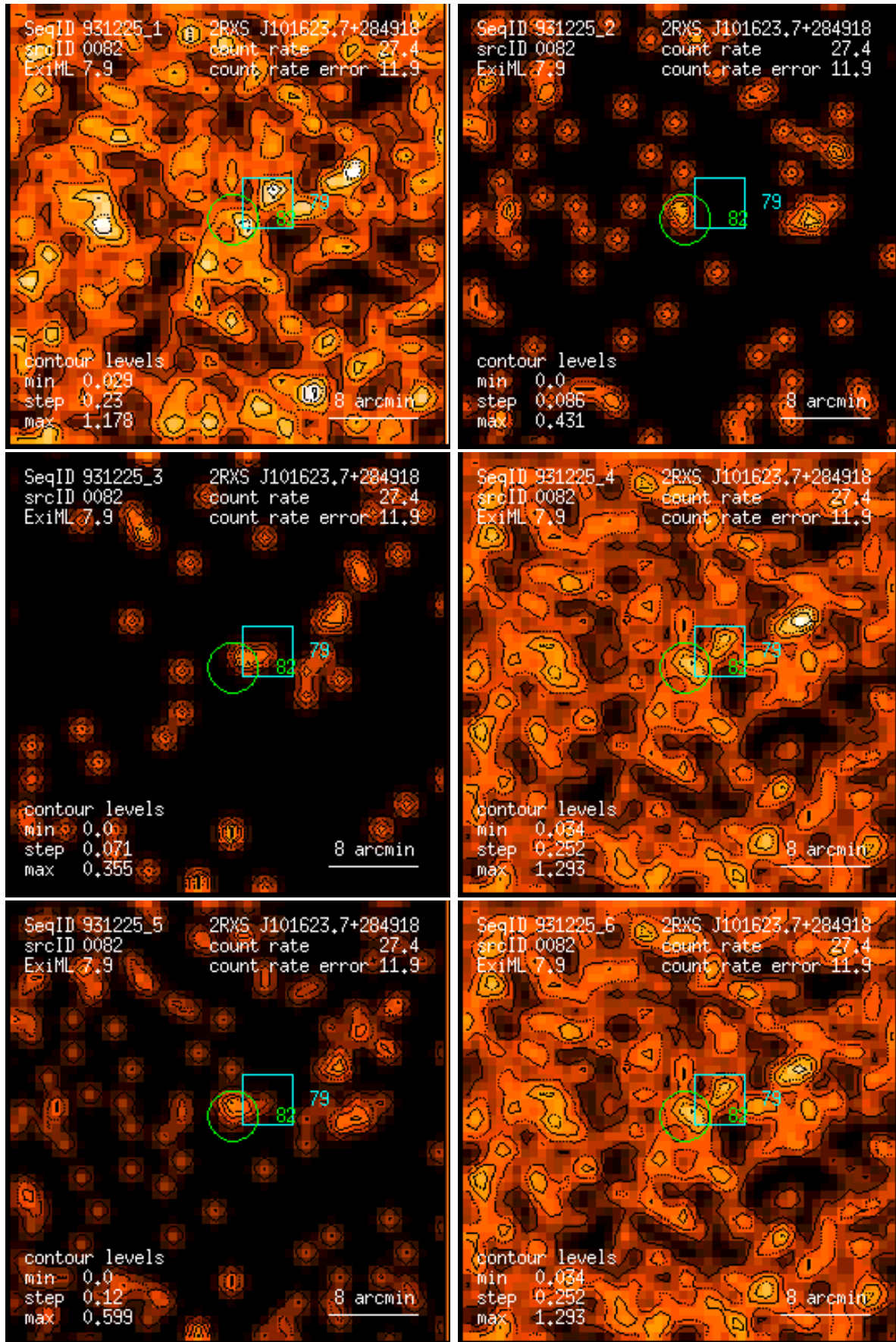
Figure 82: RASS 931225: detection 0082: band rate images, Gaussian filter: (1) PSPC channels 11 – 41, (2) 52 – 90, (3) 91 – 201, (4) 11 – 235, (5) 52 – 201, (6) 11 – 201. Broad band rates in counts/ks. Band rate contour levels in counts/ks/arcmin 2 .
