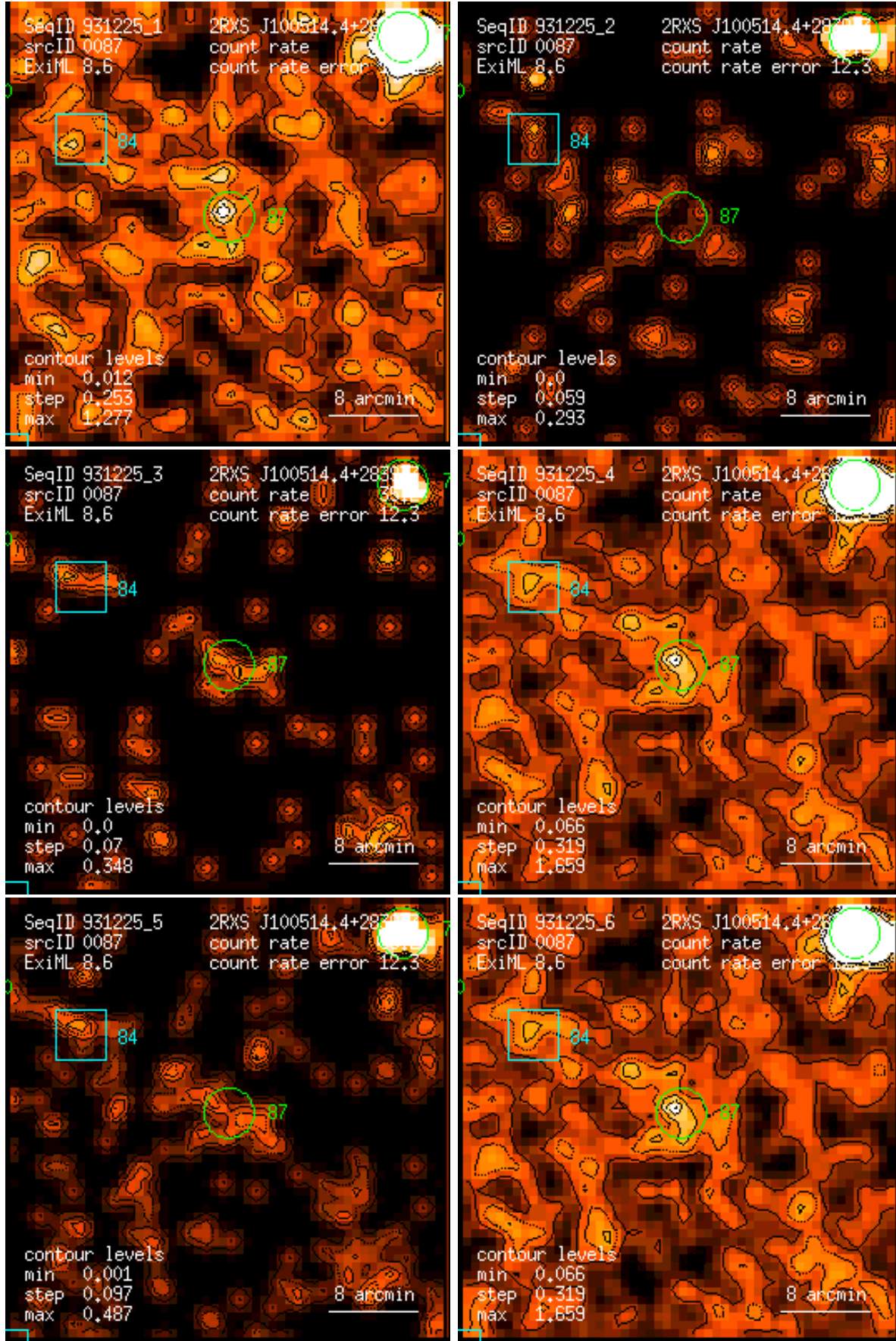
Figure 87: RASS 931225: detection 0087: band rate images, Gaussian filter: (1) PSPC channels 11 – 41, (2) 52 – 90, (3) 91 – 201, (4) 11 – 235, (5) 52 – 201, (6) 11 – 201. Broad band rates in counts/ks. Band rate contour levels in counts/ks/arcmin 2 .
