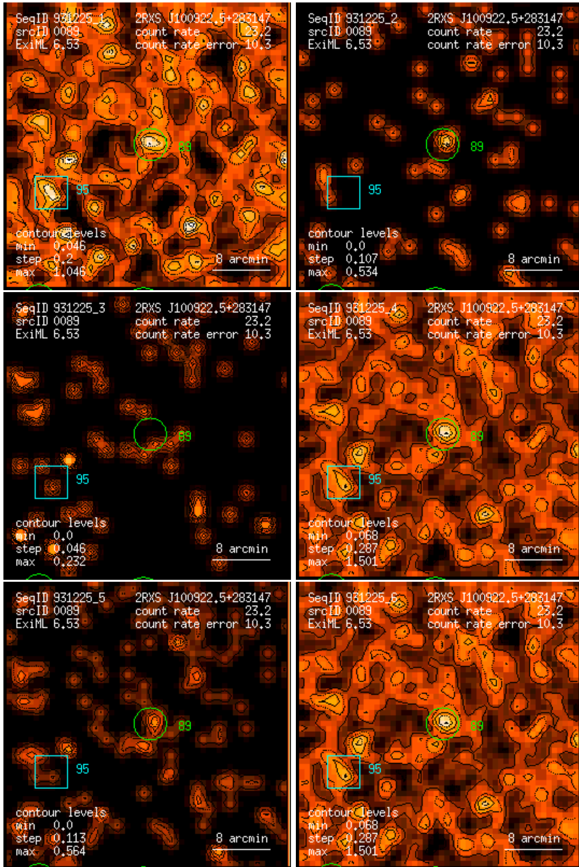
Figure 89: RASS 931225: detection 0089: band rate images, Gaussian filter: (1) PSPC channels 11 – 41, (2) 52 – 90, (3) 91 – 201, (4) 11 – 235, (5) 52 – 201, (6) 11 – 201. Broad band rates in counts/ks. Band rate contour levels in counts/ks/arcmin 2 .
