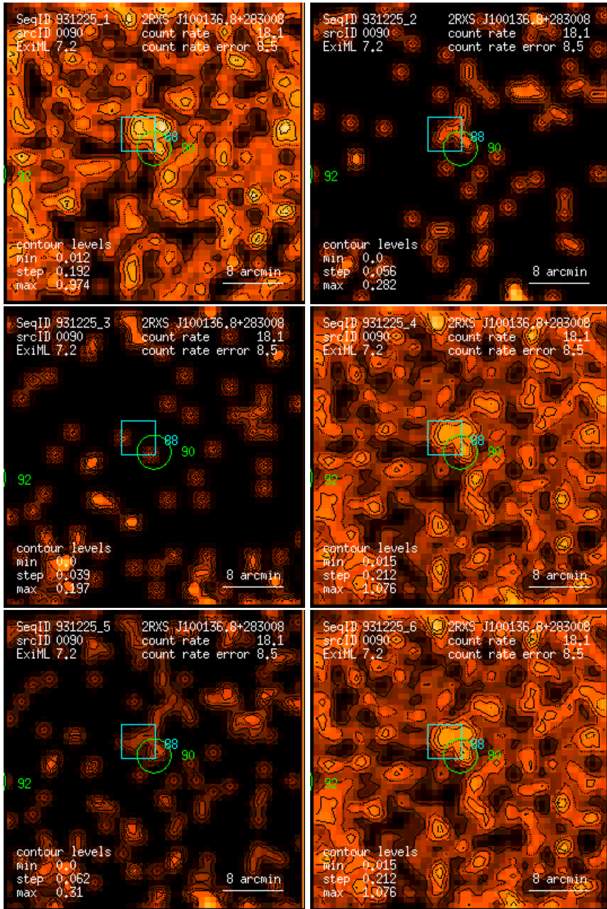
Figure 90: RASS 931225: detection 0090: band rate images, Gaussian filter: (1) PSPC channels 11 – 41, (2) 52 – 90, (3) 91 – 201, (4) 11 – 235, (5) 52 – 201, (6) 11 – 201. Broad band rates in counts/ks. Band rate contour levels in counts/ks/arcmin 2 .
