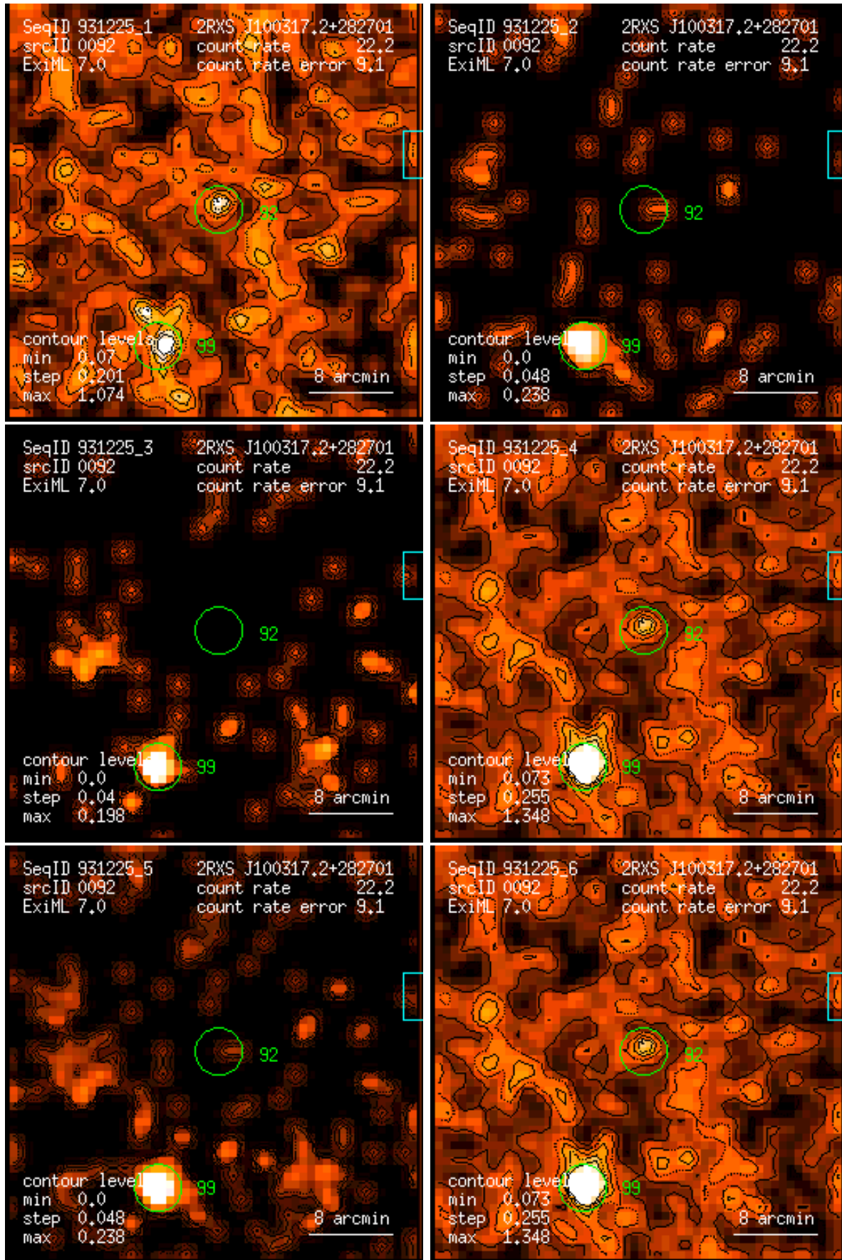
Figure 92: RASS 931225: detection 0092: band rate images, Gaussian filter: (1) PSPC channels 11 – 41, (2) 52 – 90, (3) 91 – 201, (4) 11 – 235, (5) 52 – 201, (6) 11 – 201. Broad band rates in counts/ks. Band rate contour levels in counts/ks/arcmin 2 .
